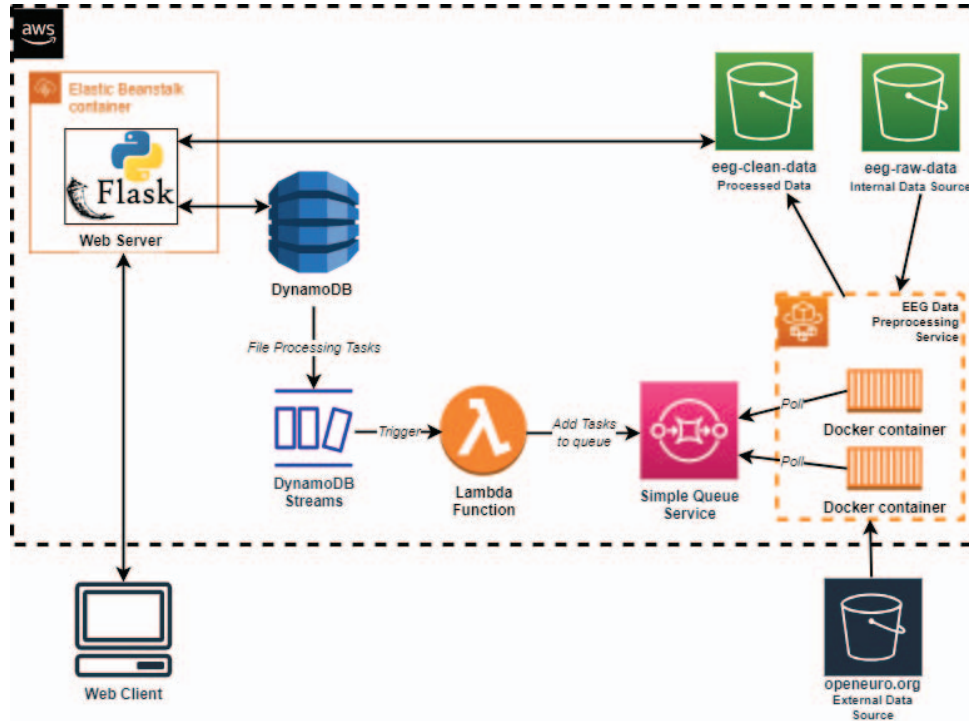
Fig. 2: Serverless EEG Data Preprocessor Framework
