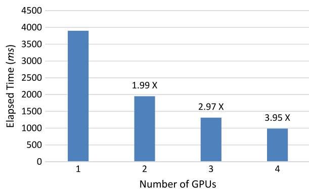
Fig. 9. Computational time and speedup of GPU-AxT implementation using multiple Tesla C2070 GPUs on a molecular system with 8000 particles. The elapsed time is the average iteration time over 100 runs.
