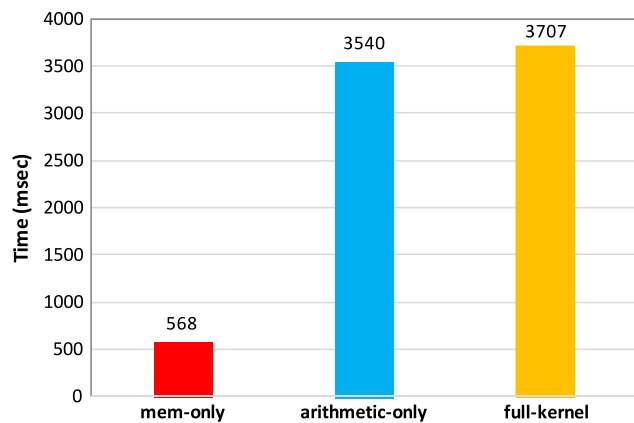
Fig. 6. Memory-only, arithmetic-only, and full-kernel time in GPU-AxT on a system with 3375 particles. 70.6% of memory operations are overlapped with arithmetic operations.
