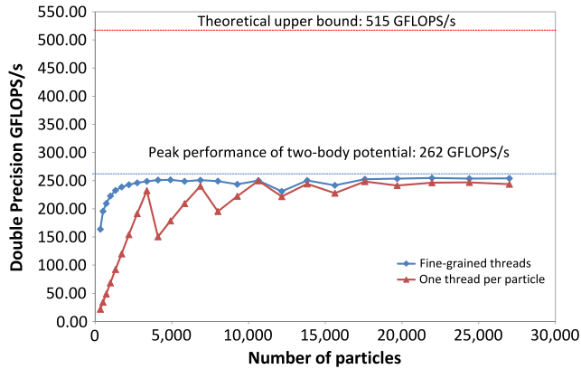
Fig. 5. Performance comparison of GPU-AxT implementations on systems of various sizes in terms of double-precision floating point throughput on NVIDIA Tesla C2070.
