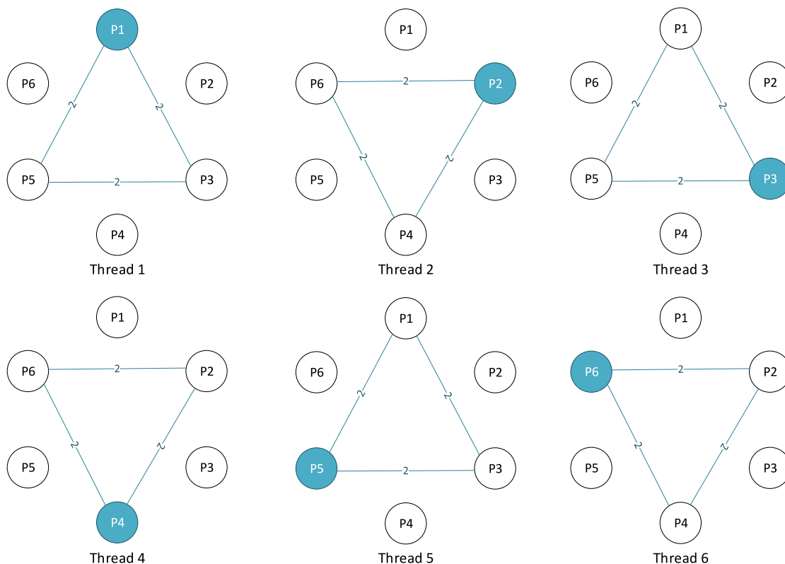
Fig. 3. Order three rotational symmetry in a system with 6 particles. The highlighted particle is the first particle a thread handles. Threads 1, 3, 5 over calculate triplet (P1, P3, P5) while threads 2, 4, 6 over calculate triplet (P2, P4, P6).
