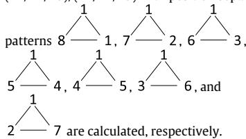
Fig. 2. An example of enumerating triplets without sharing rotational symmetry in position separation patterns by the first thread (thread 1) in a system with 10 particles.
