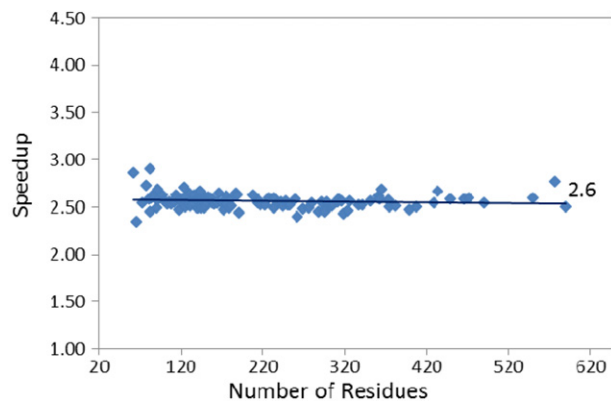
Fig. 8. Performance of the balanced GPU-CSSP with respect to the unbalanced GPU-CSSP on Tesla C2070.
