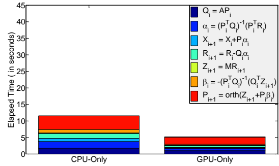
Figure 7: Comparison of the average elapsed computational time per iteration for different steps in BCG on CPU and GPU processors when eigendecomposition on Z^T Z is used to replace QR decomposition on Z to obtain orthogonal new search direction matrix P_{i+1}
