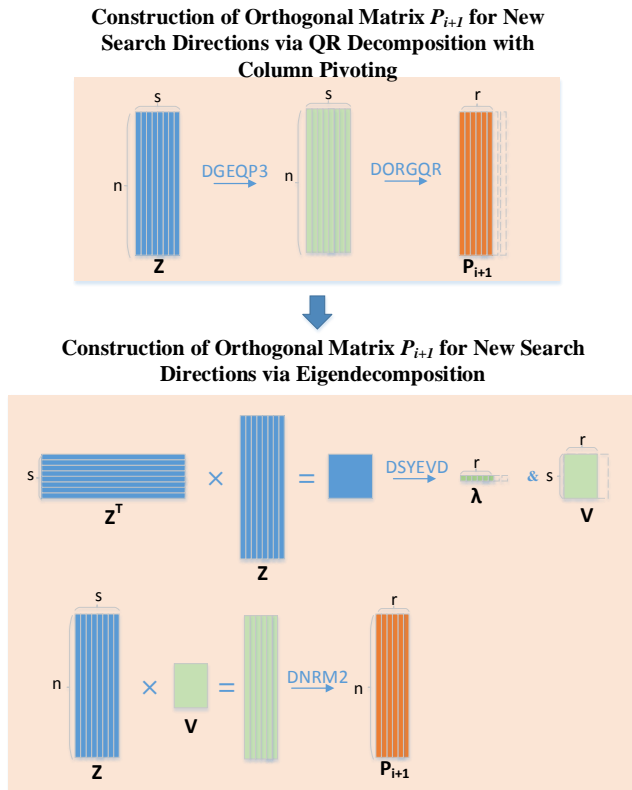
Figure 6: Eigendecomposition on Z^T Z to replace QR decomposition on Z to obtain orthogonal new search direction matrix P_{i+1}
