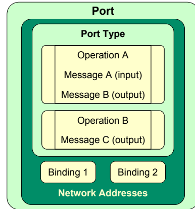
Figure 1: Cascading Elements of the WSDL
