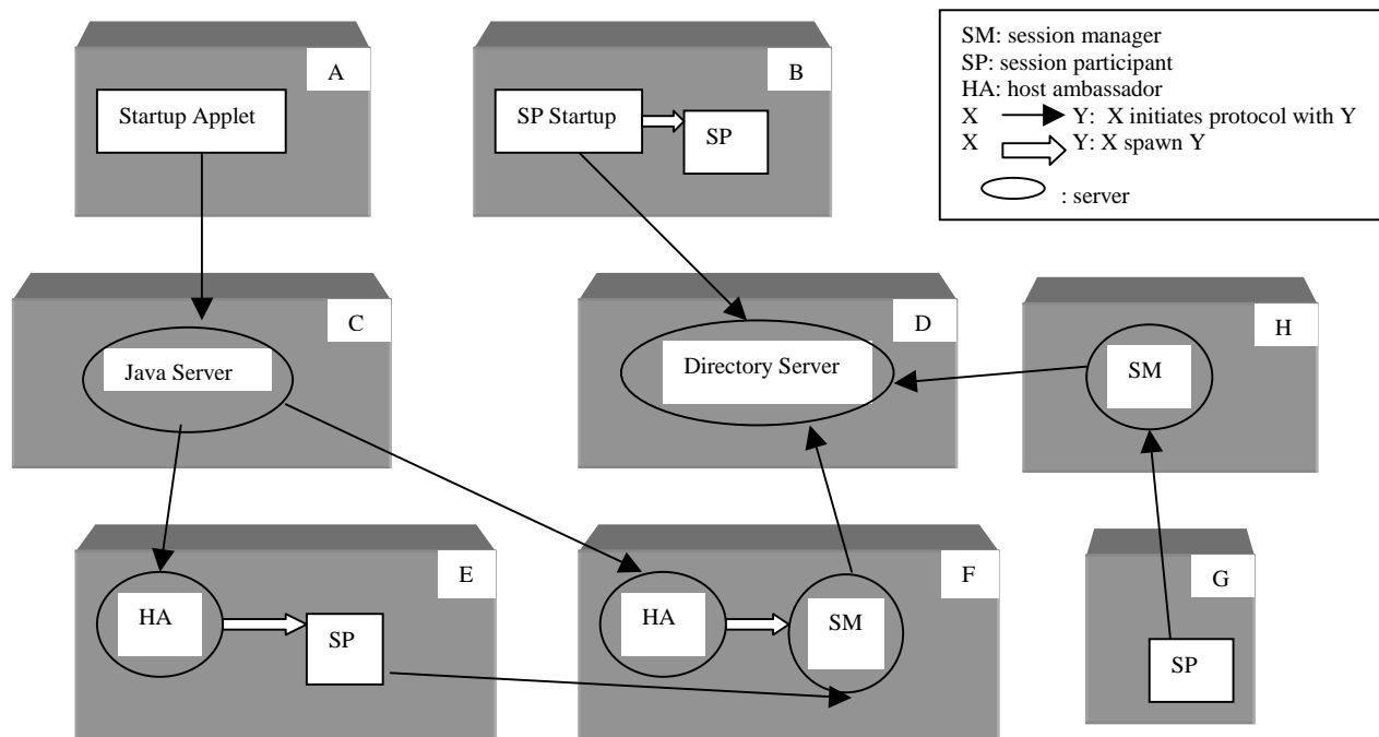
Figure 3: Various IRI-h session startup scenarios
