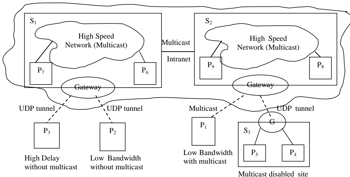
Figure 1: A Typical IRI-h Network Structure
