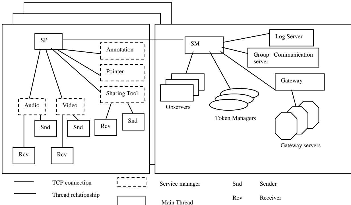
Figure 2: IRI-h Software Architecture
