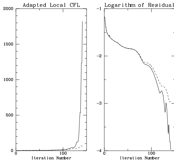
FIGURE 1. CFL and steady-state residual versus iteration count for defect correction and Newton-Krylov solvers.
