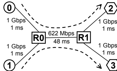
Fig. 1. Network Topology
