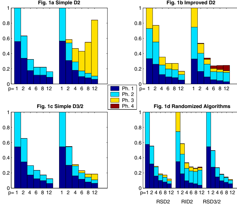
Fig. 1. a-c: Relative performance of deterministic algorithms on graphs fe144 (left-half on each subgraph) and ev02 (right-half). Fig. 1d: Relative performance of randomized algorithms on ev02.
