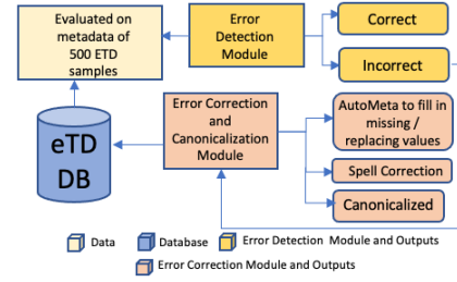
Fig. 1. MetaEnhance Framework.
