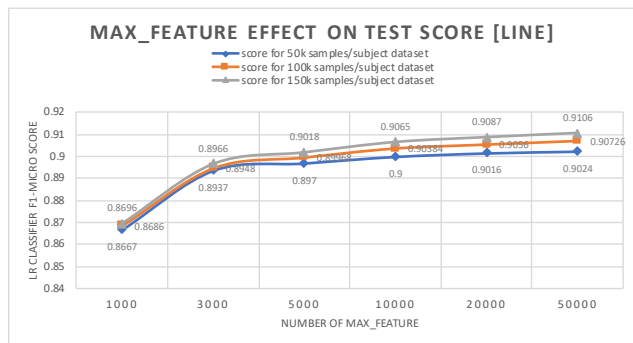
Fig. 2. Performance changes with d_f for LR.
