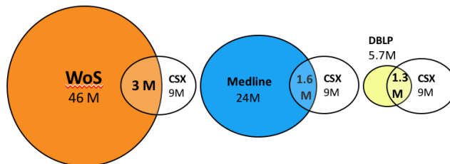
Fig. 1. Matching results between CiteSeerX (CSX) and reference datasets.
