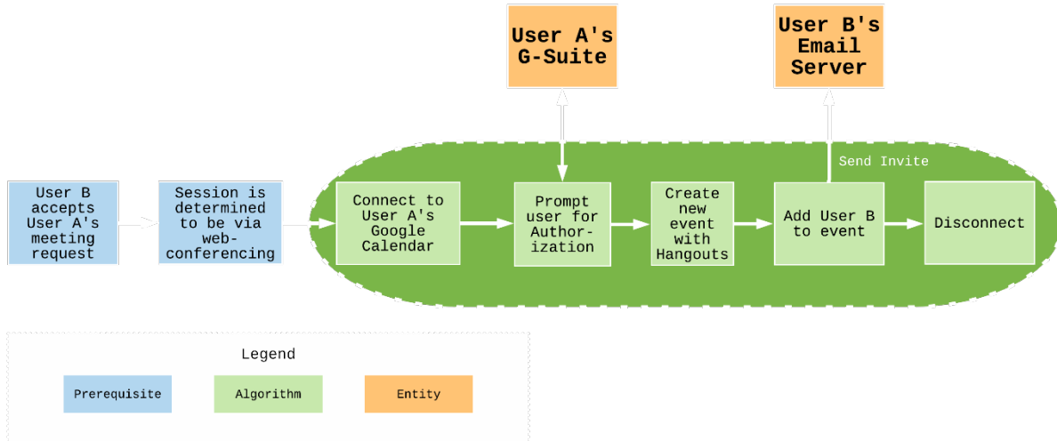
FIGURE 17 - WEB-CONFERENCE APPOINTMENT CREATOR ALGORITHM FLOW confirmation.
