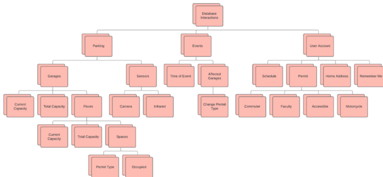
Figure 2. Database Interactions
