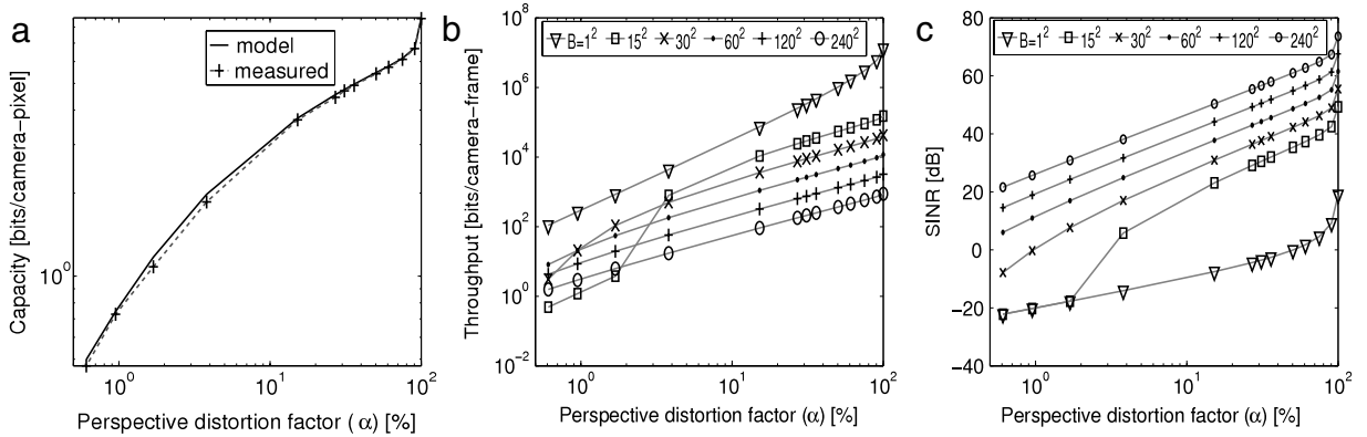
Fig. 6. (a) Capacity in bits/camera pixel ( C_{\text{camera-pixel}}(\alpha) ) for different perspective scaling ( \alpha ) of screen image on camera (b) Throughput in bits/frame vs. \alpha for different block sizes (1 frame = R_{\text{cam}} pixels, B = 15^2 means 15 \times 15 pixel block on screen) (c) SINR per block vs. \alpha for different block sizes B .
