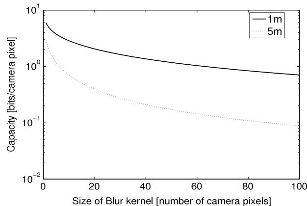
Fig. 8. Capacity vs. blur.
