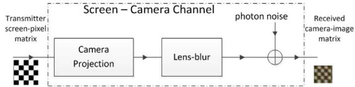
Fig. 2. Screen-camera channel model.
