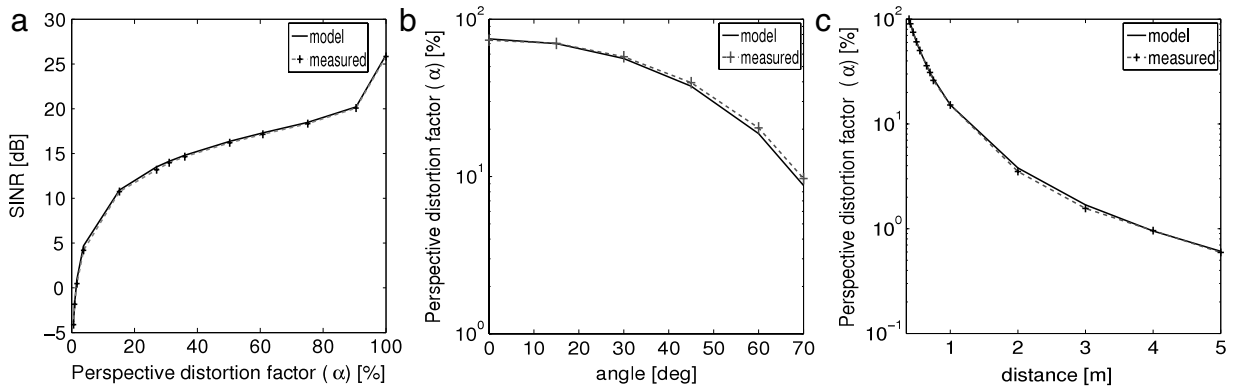
Fig. 7. (a) SINR for different perspective scaling ( \alpha ) of screen image on camera (b) Perspective distortion \alpha vs. angle between screen and camera (c) Perspective distortion factor \alpha vs. distance between screen and camera.
