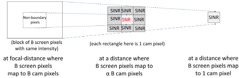
Fig. 4. Illustration of interference between pixel-blocks due to perspective distortion for SINR computation.
