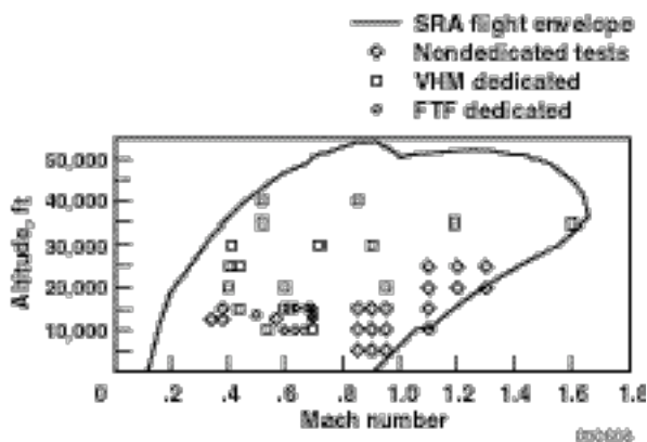
Figure 5. Flight envelope.
