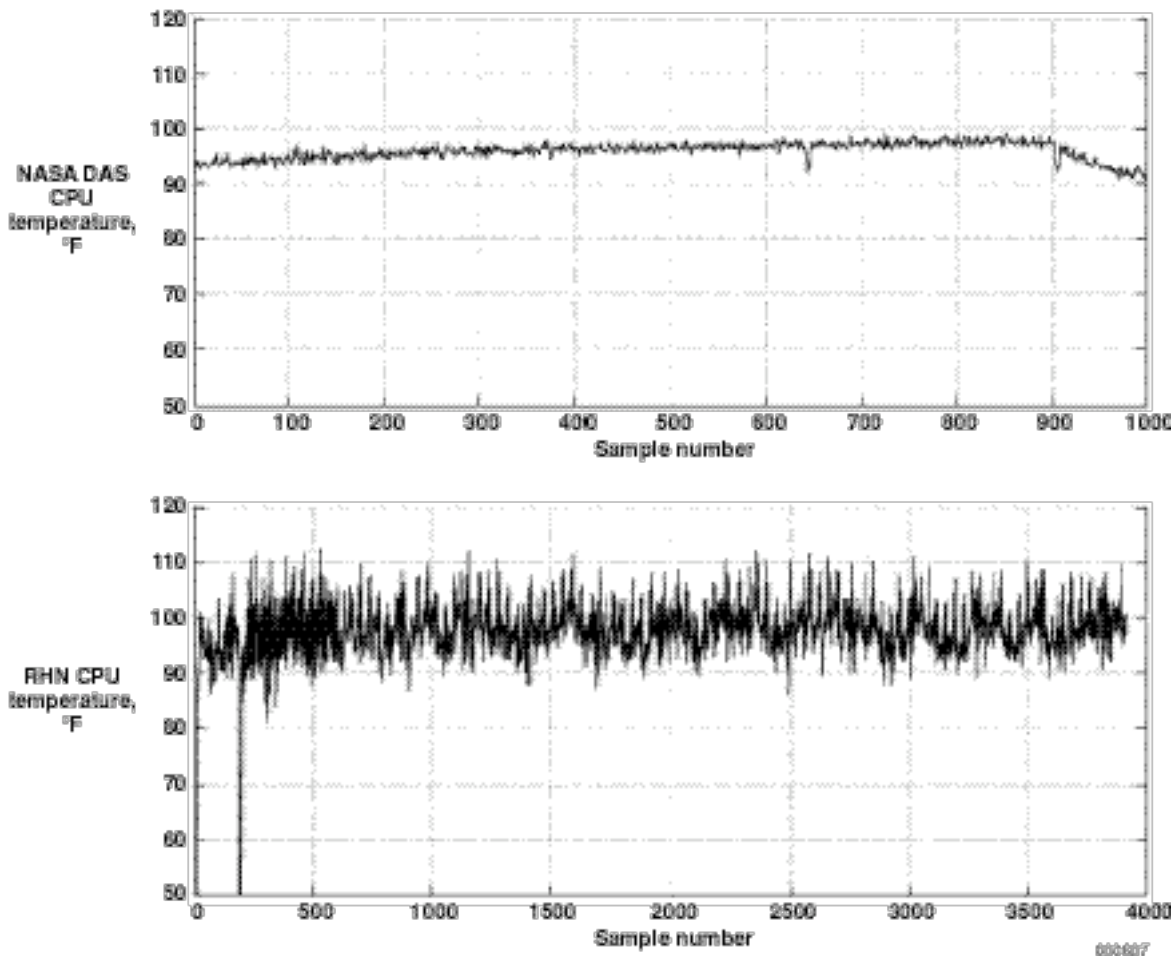
Figure 6. Flight data.
