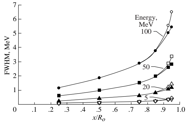
Figure 2. Full width at half maximum (FWHM) of energy distribution of monoenergetic proton beam as function of scaled depth in aluminum. Upper curves near end of range refer to Payne's method; lower curves are modified widths.
