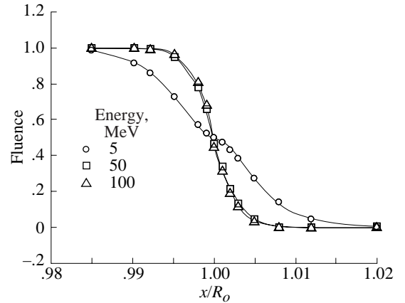
Figure 3. Total particle fluence of proton beam in aluminum near maximum range as function of beam energy.
