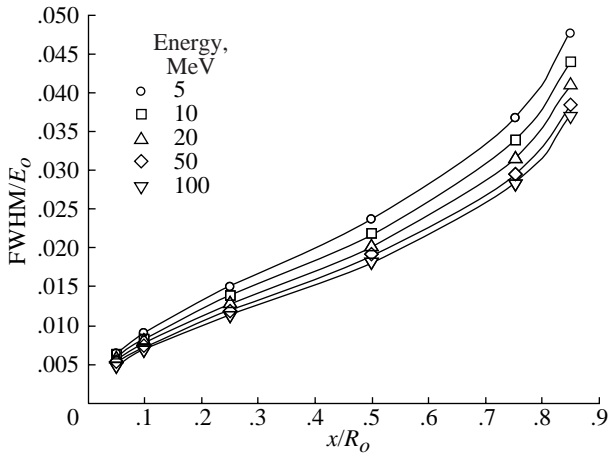
Figure 1. Energy scaled full width at half maximum (FWHM) of energy distribution of monoenergetic proton beam as function of scaled range in liquid oxygen.
