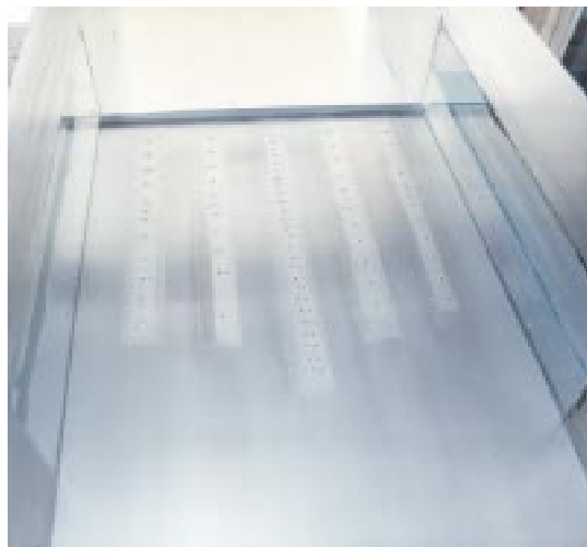
Figure 2. MSU Separated Flow Generator Model in SBRT. Note Microphones, Pressure Taps, and DPIV Windows.
