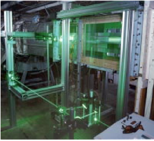
Figure 4. DPIV Laser Optics System in SBRT.
