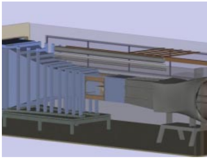
Figure 1. NASA Langley Subsonic Basic Research Tunnel.
