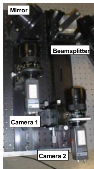
Figure 7. Recording System Receiver Configuration.
