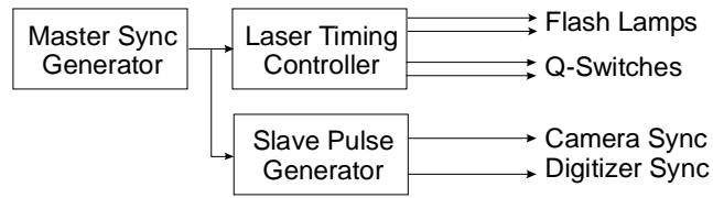
Figure 9. Laser / Camera Synchronization.
