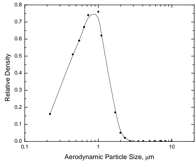
Figure 5. DEHS Nominal Particle Size Distribution.
