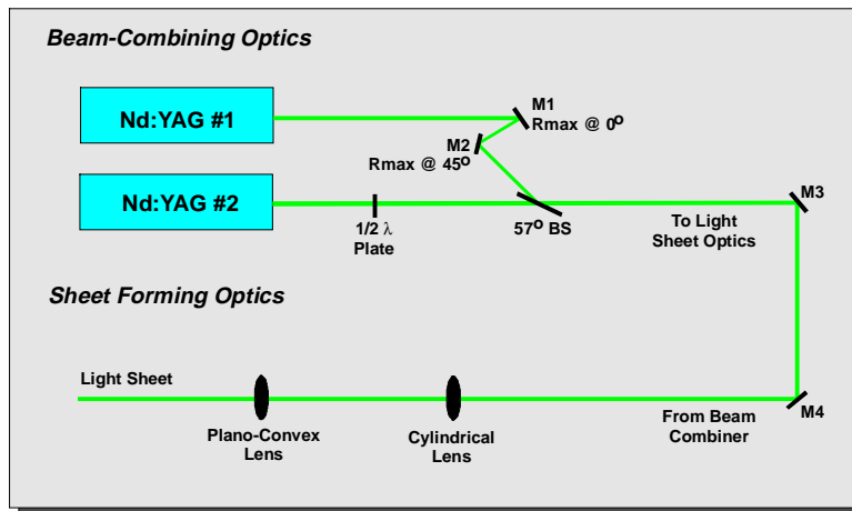
Figure 3. DPIV Laser Optics System.
