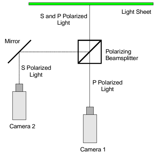
Figure 8. Polarization Separation Concept.
