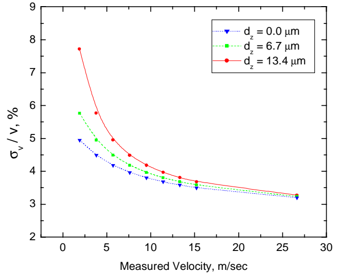
Figure 11. Velocity Uncertainty Estimates.
