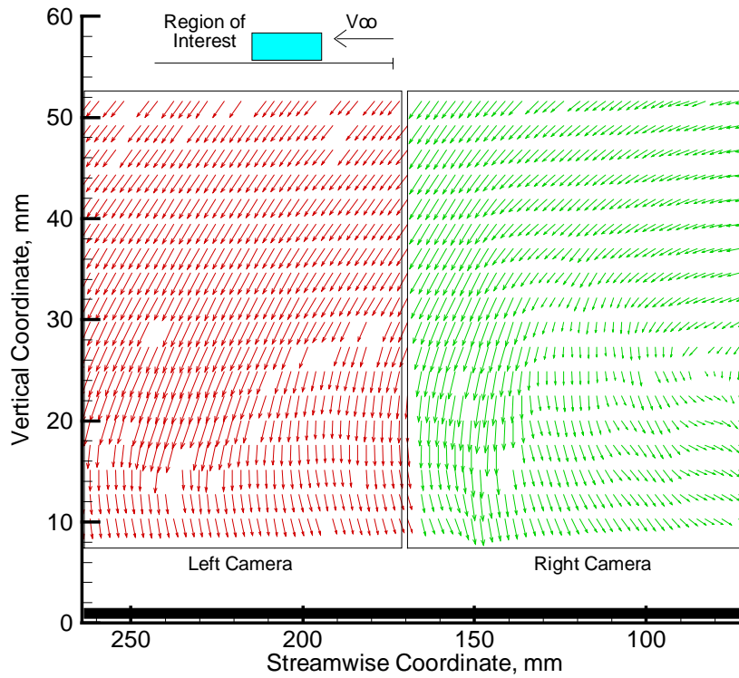
Figure 12. Representative Separated Flow Data Obtained Downstream of Splitter Plate Leading Edge Fence.
