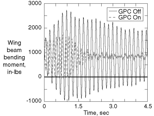
Figure 10. - Effect of GPC on damped response of wing beam bending mode at 120 kt for \delta_3 = -15^\circ .
