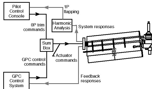
Figure 5. - Schematic of active stability control system.
