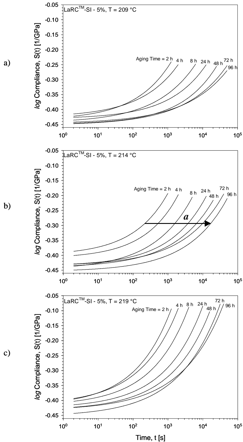
Figure 4. Creep compliance momentary curves plotted as a function of time for the three test temperatures: a) T=209°C, b) T=214°C, c) T=219°C at 5% molecular weight offset. The creep compliance momentary curves are shifted to coincide with the 96 h ageing time reference curve.
