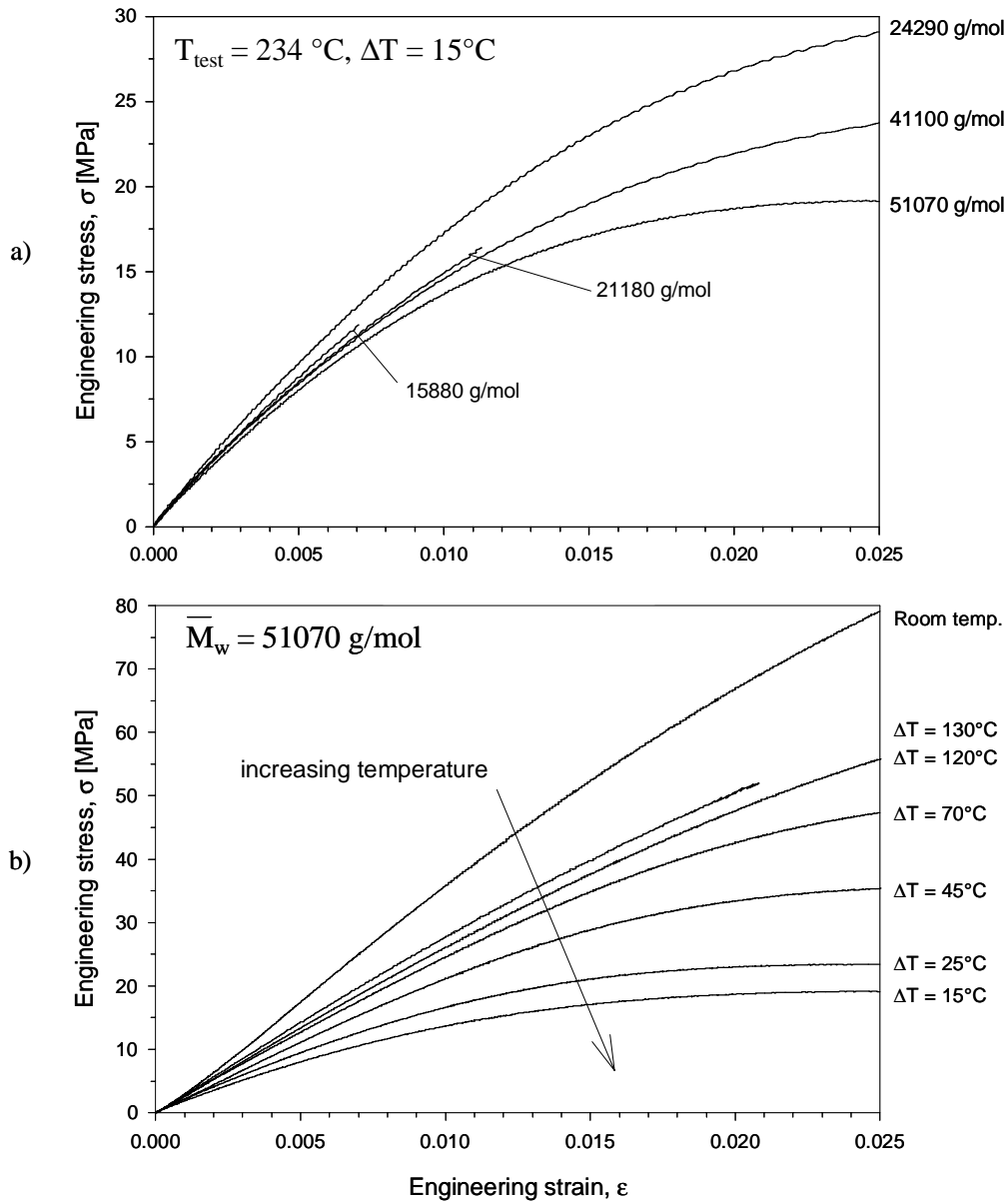
Figure 1. Stress-strain curves for unnotched specimens: (a) of different molecular weights at a reduced test temperature of 15^\circ\text{C} below T_g ; and (b) of high molecular weight ( \bar{M}_w = 51070 \text{ g/mol} ) displaying the effects of different reduced temperatures. Each curve represents a single test specimen. Curves that terminate before the 2.5% strain level indicate failure.
