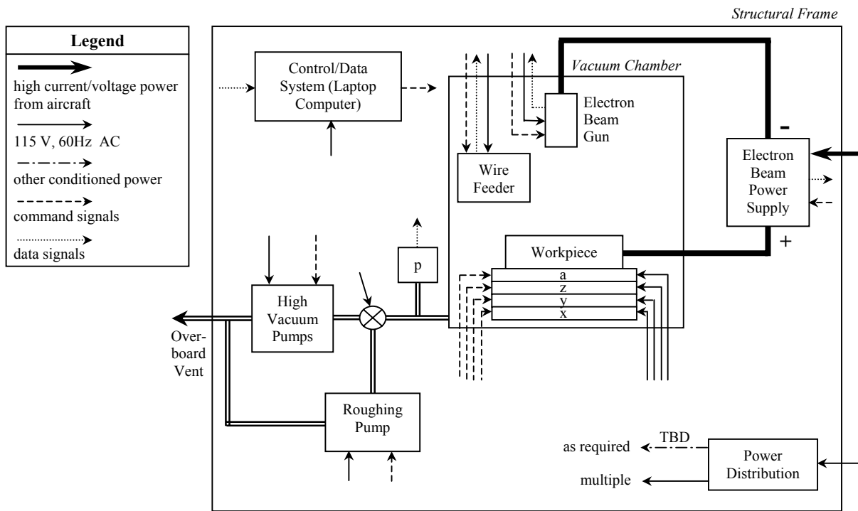
Figure 2. Schematic diagram of low-voltage EB F 3 system.
