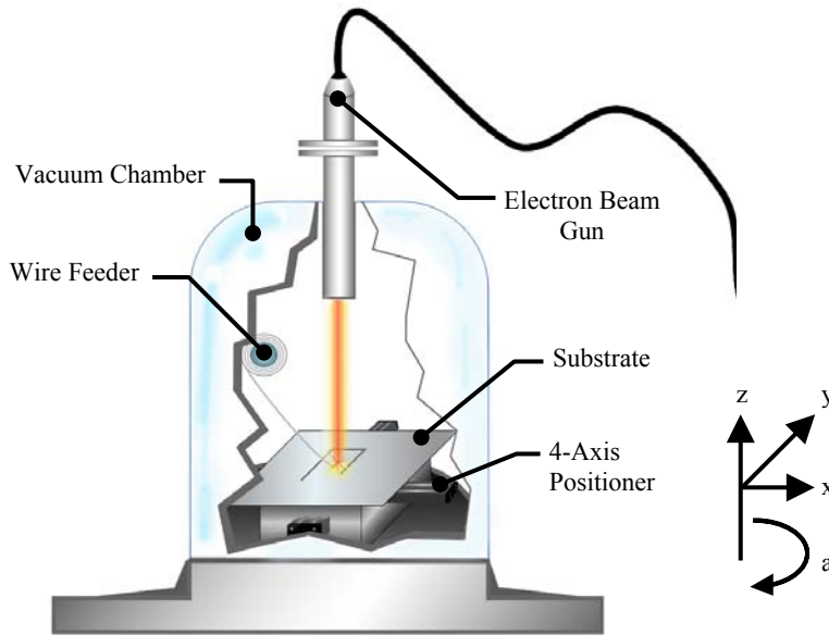
Figure 1. Artist's conception of low-voltage EB F 3 system.
