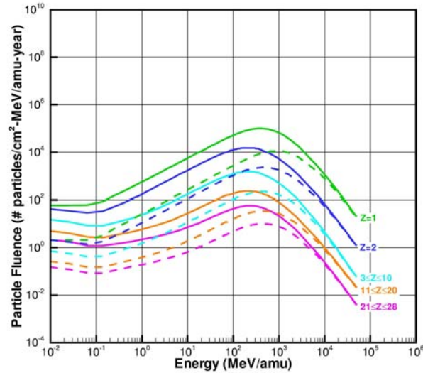
Fig. 2. Galactic cosmic ray spectra at the 1977 Solar Minimum (full lines) and 1990 Solar Maximum (dashed lines) according to Badhwar et al.
