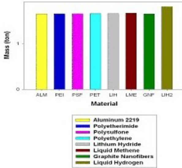
Fig. 10. Optimized mass for Lunar reference and trade missions for various materials.
