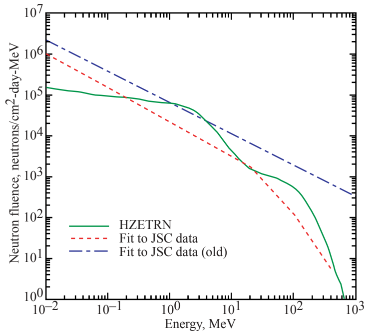
Figure 15. The neutron environment of STS-31 (28.5° inclination, 617 km) on Apr. 24–29, 1990 predicted by current model compared to JSC data (Keith et al. 1992).
