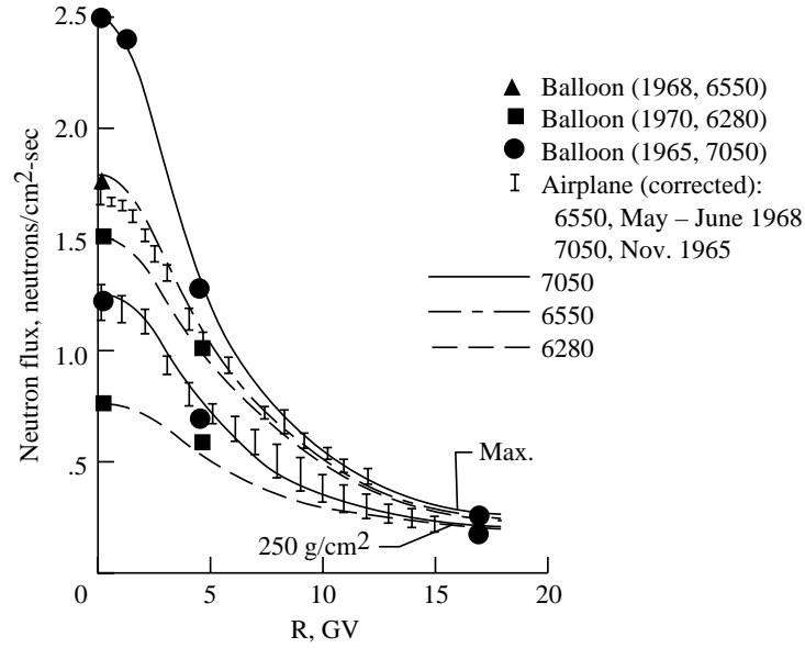
Figure 11. Fast neutron flux (in the range from 1 to 10 MeV) at the transition maximum and 250 g/cm 2 depth as a function of vertical cutoff rigidity R for various times in the solar cycle and Deep River Neutron Monitor (DRNM) count rates.
