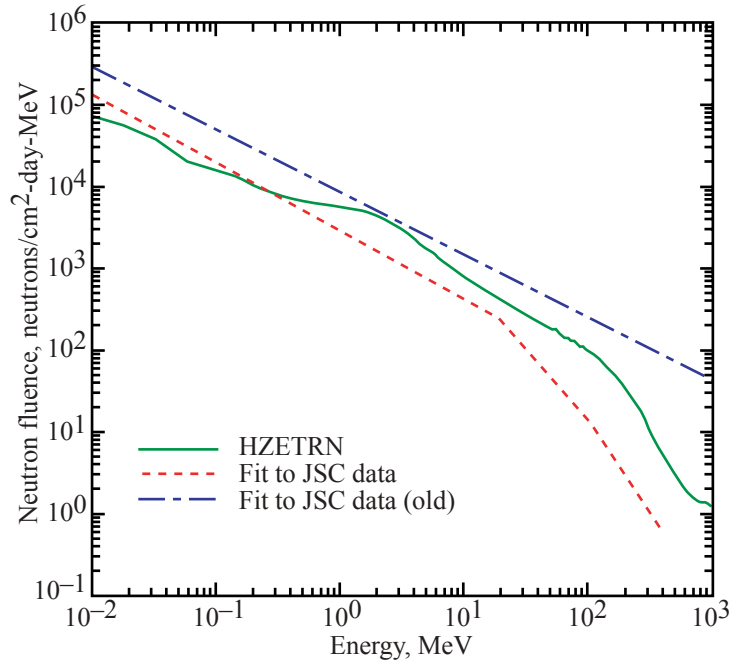
Figure 14. The neutron environment of STS-36 (62° inclination, 246 km) on Feb. 28–Mar. 3, 1990 predicted by current model compared to Johnson Space Center (JSC) data (Keith et al. 1992).
