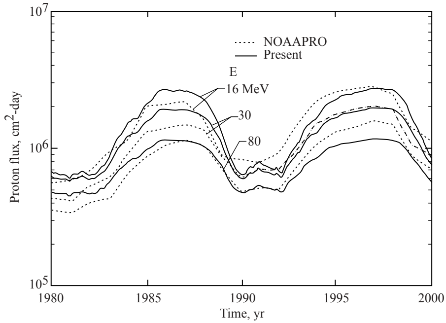
Figure 10. Predicted proton flux levels of the present model and those of the NOAAPRO model.
