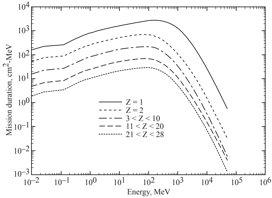
Figure 3. Galactic cosmic ray (GCR) environment for first week of June 2001 outside the geomagnetic field; ISS GCR free space, 400 \text{ km} \times 51.6^\circ .
