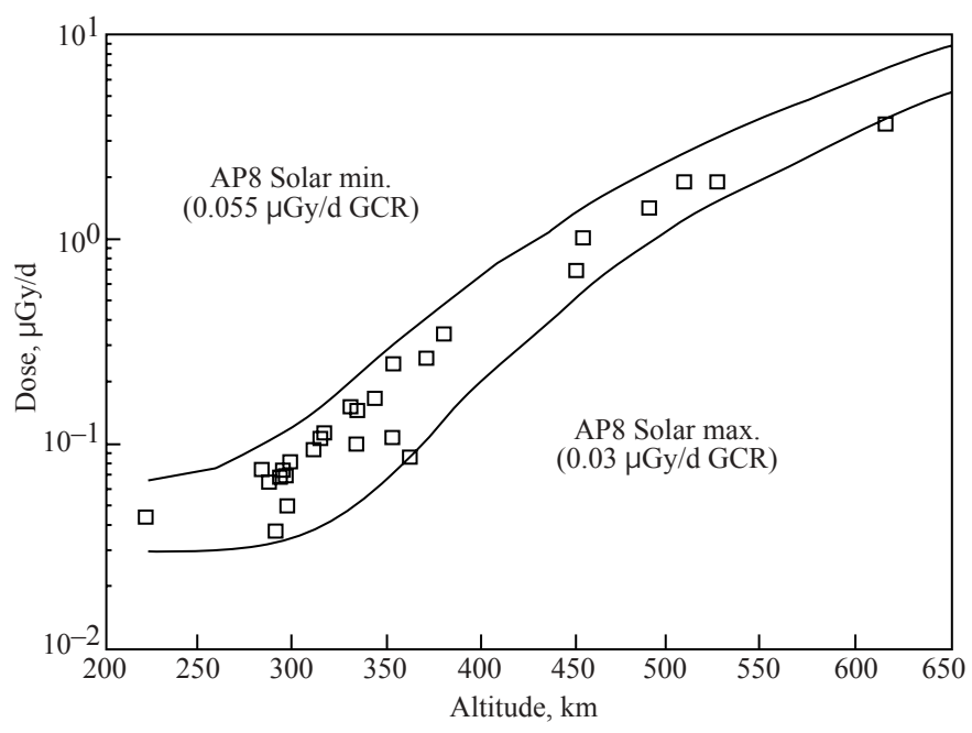
Figure 5. Shuttle measurements in low inclination, low Earth orbit (LEO) compared to model calculations (Atwell et al. 1989).
