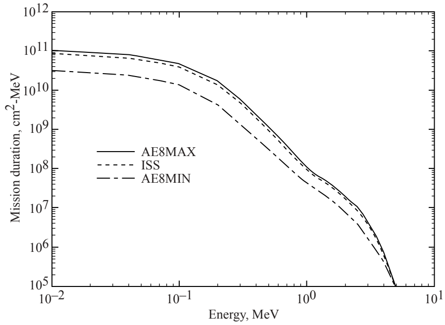
Figure 7. ISS electron differential spectrum for first week of June 2001; 400 \text{ km} \times 51.6^\circ .
