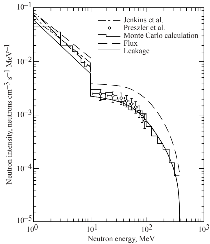
Figure 12. Neutron intensity at top of Earth's atmosphere over Palestine, TX during September 1971 according to various models and experiments.
