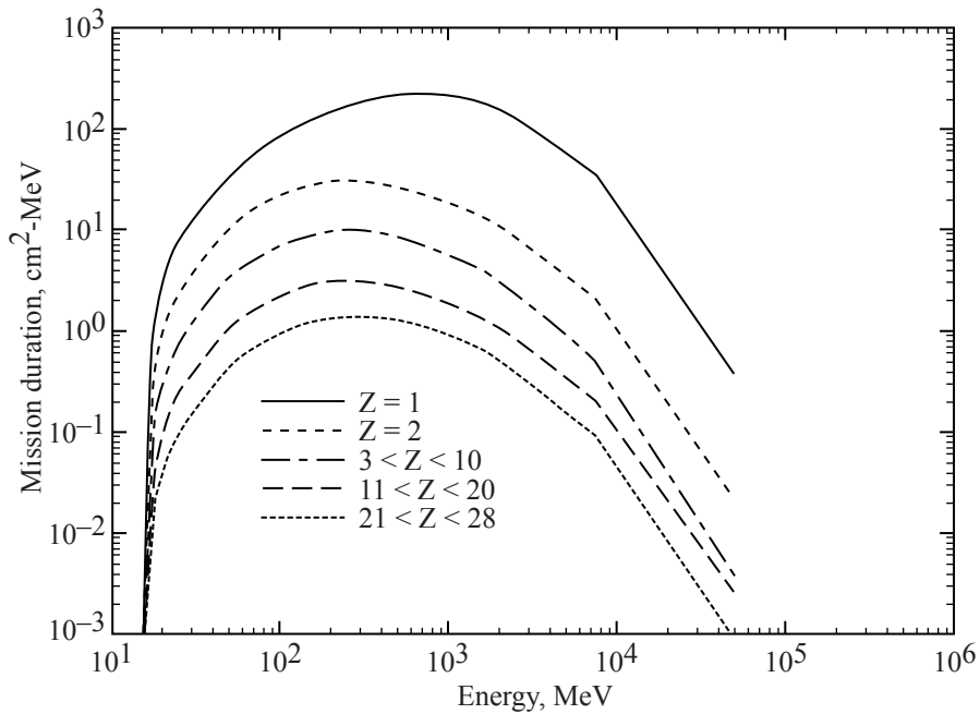
Figure 4. ISS GCR environment in first week of June 2001 according to the present model; ISS GCR + cutoff field; 400 \text{ km} \times 51.6^\circ .
