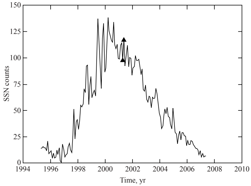
Figure 1. Sunspot number (SSN) for International Space Station (ISS) environment in first week of June 2001 according to present model; 400 \text{ km} \times 51.6^\circ .
