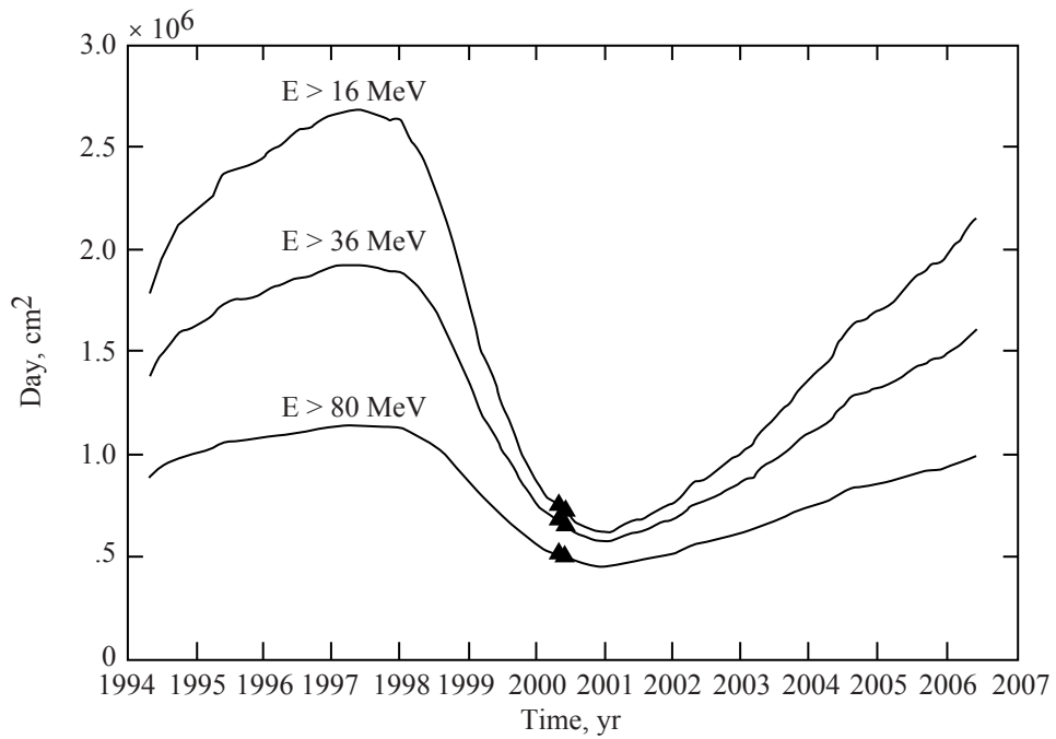
Figure 8. ISS proton environment for first week of June 2001; ISS trapped proton field, 400 \text{ km} \times 51.6^\circ .
