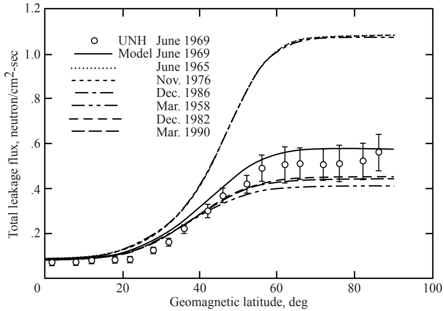
Figure 13. GCR induced neutron leakage flux for different solar cycle maxima and minima compared to measurements by University of New Hampshire by Lockwood et al.
