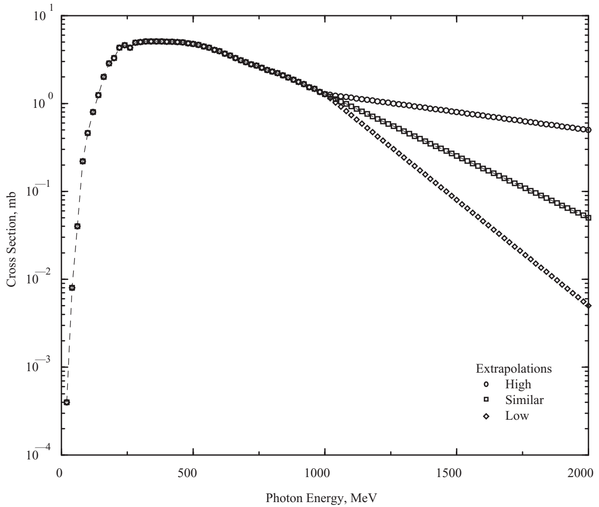
Figure 2. Photofission cross section for ^{209}\text{Bi} .
