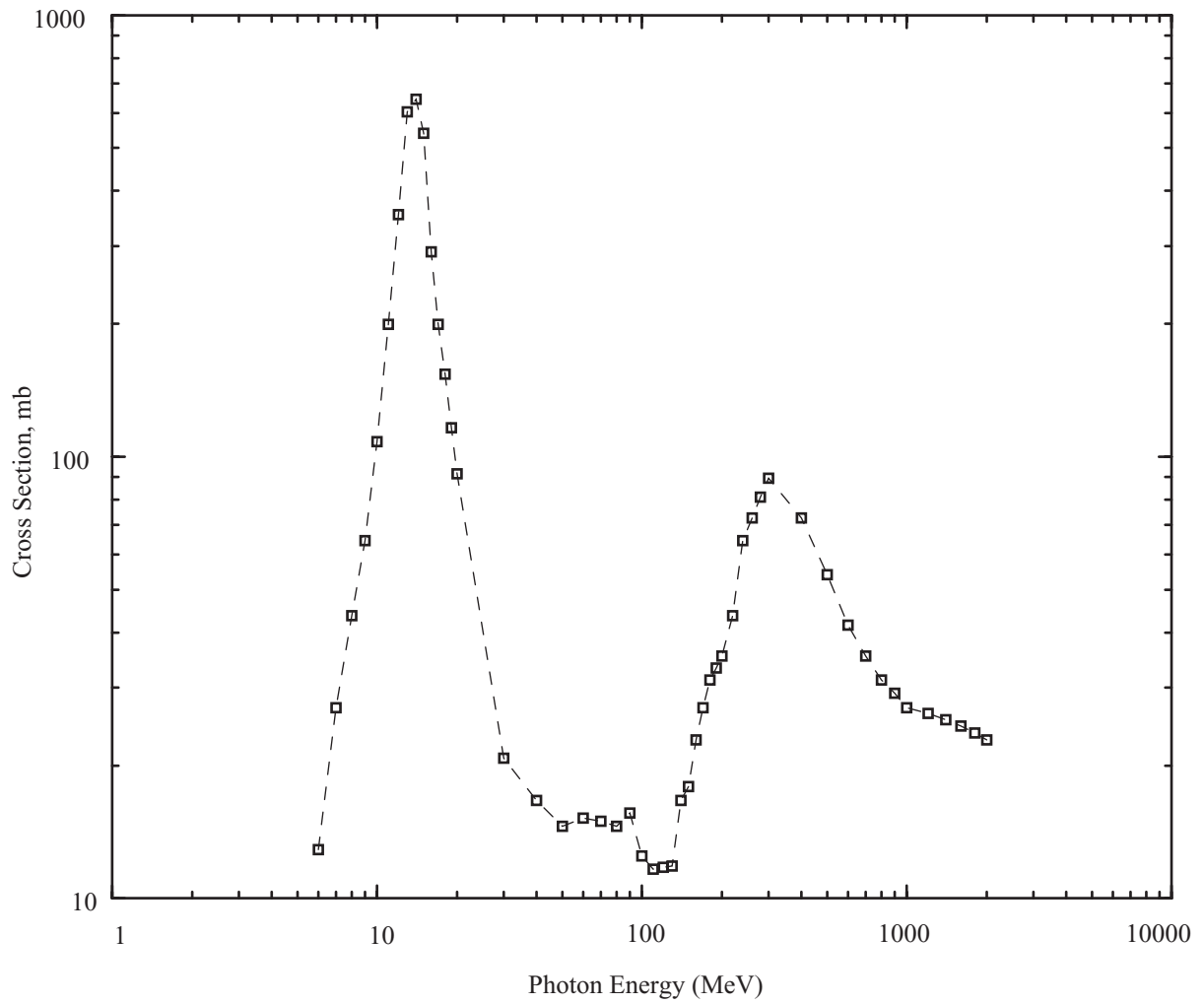
Figure 3. Photoabsorption cross section for ^{208}\text{Pb} .
