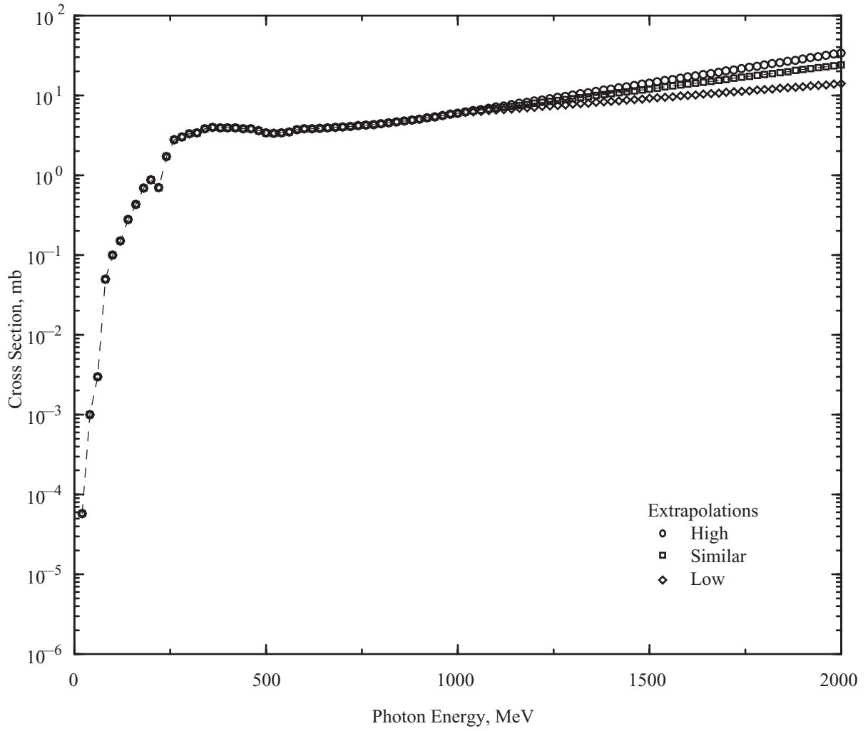
Figure 1. Photofission cross section for ^{208}\text{Pb} .
