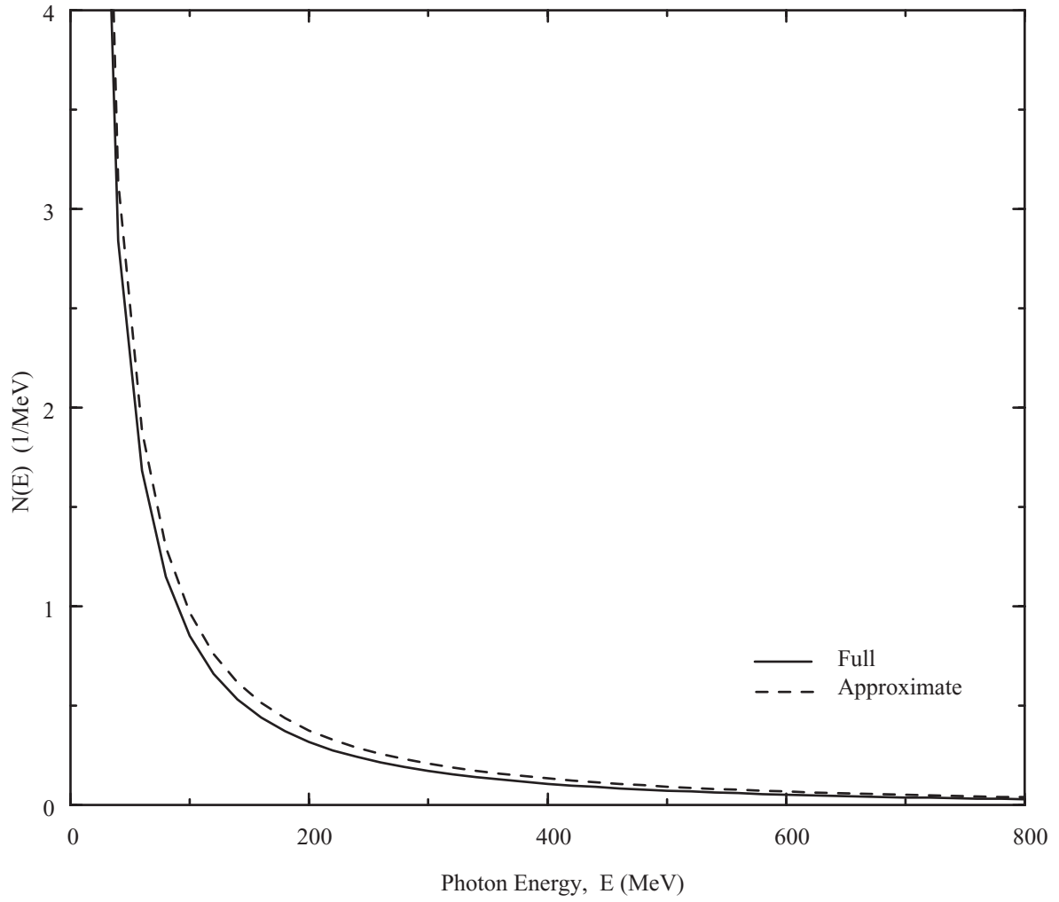
Figure 4. Comparison of the full (solid line) and approximate (dashed line) WW number spectrums per unit energy.
