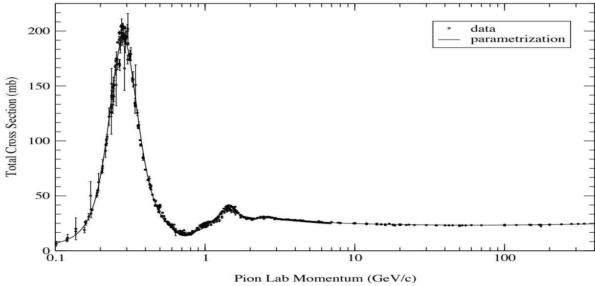
Figure 3: Data [17] plotted against the parameterization given by equations (48) and (49)
