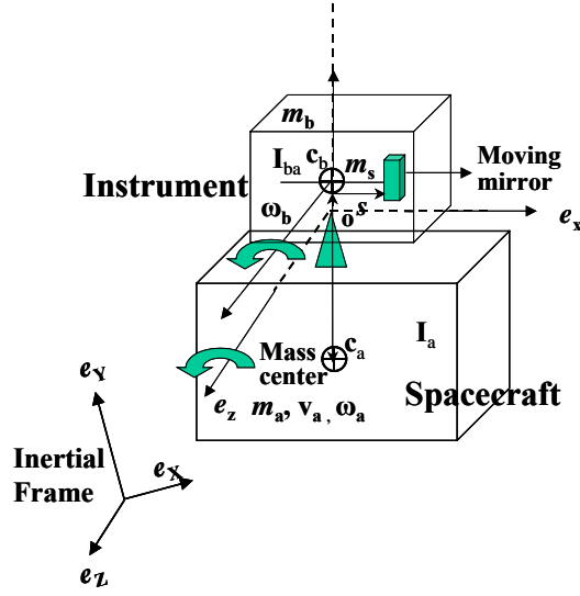
Figure 5: Body and inertia coordinates for two-rotation-axis plane motion.
