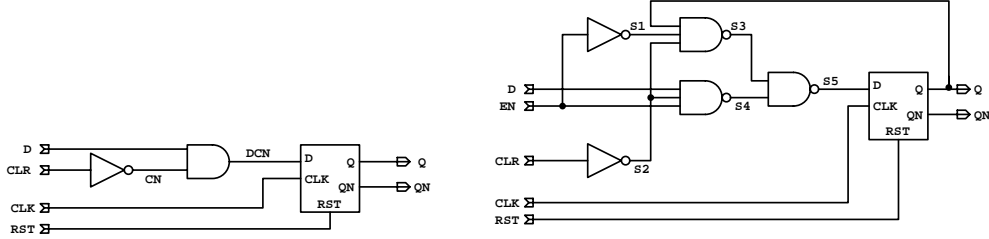
Figure 7: (a) cdfif (b) cedff
