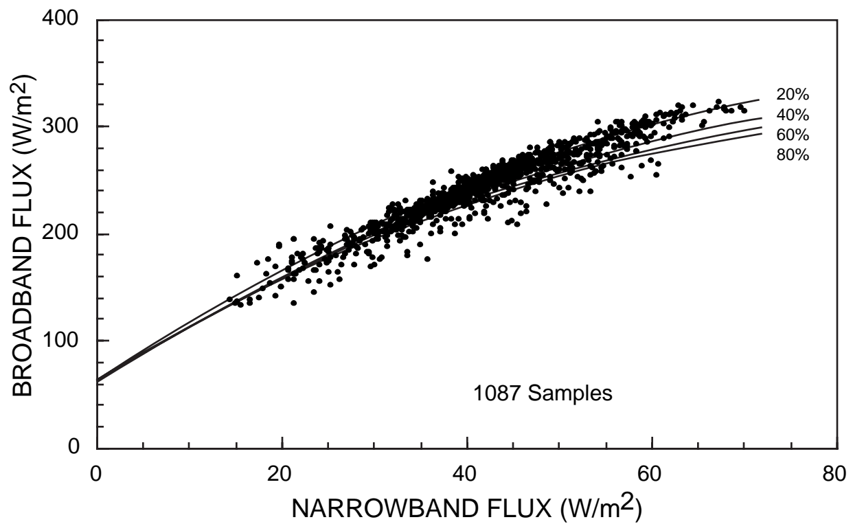
Figure 6. Correlations of ERBS LW and GOES IR fluxes for April 1985; curves indicate regression fits at particular relative humidities.
