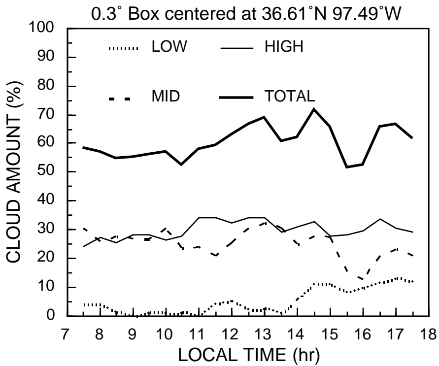
Figure 16. Mean hourly cloud amounts for 0.3° and 2.5° (average of 0.5°) regions centered on SCF for April 5 to May 1, 1994.
