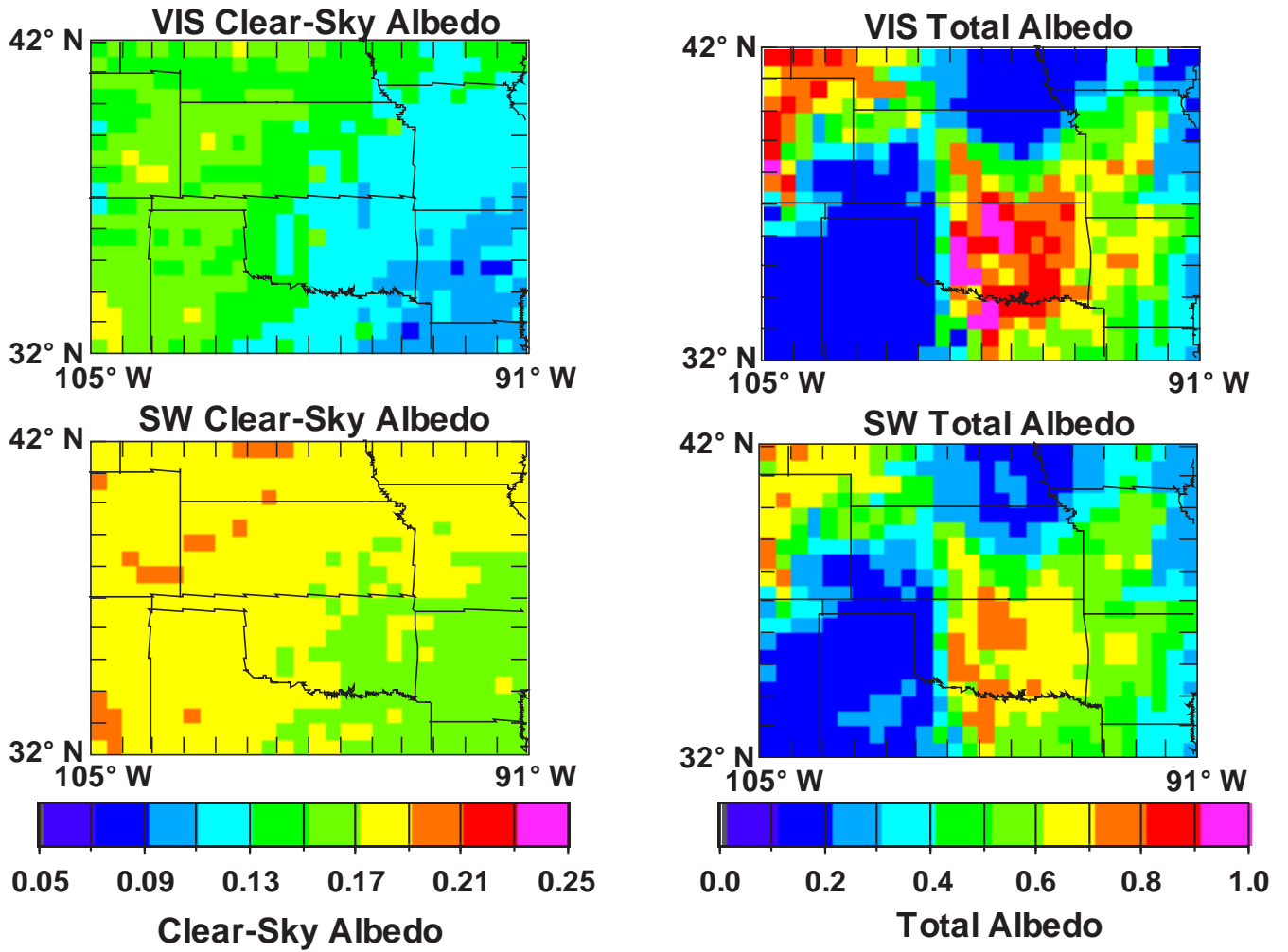
Figure 14. VIS and SW albedos for 1800 UTC, April 25, 1994.
