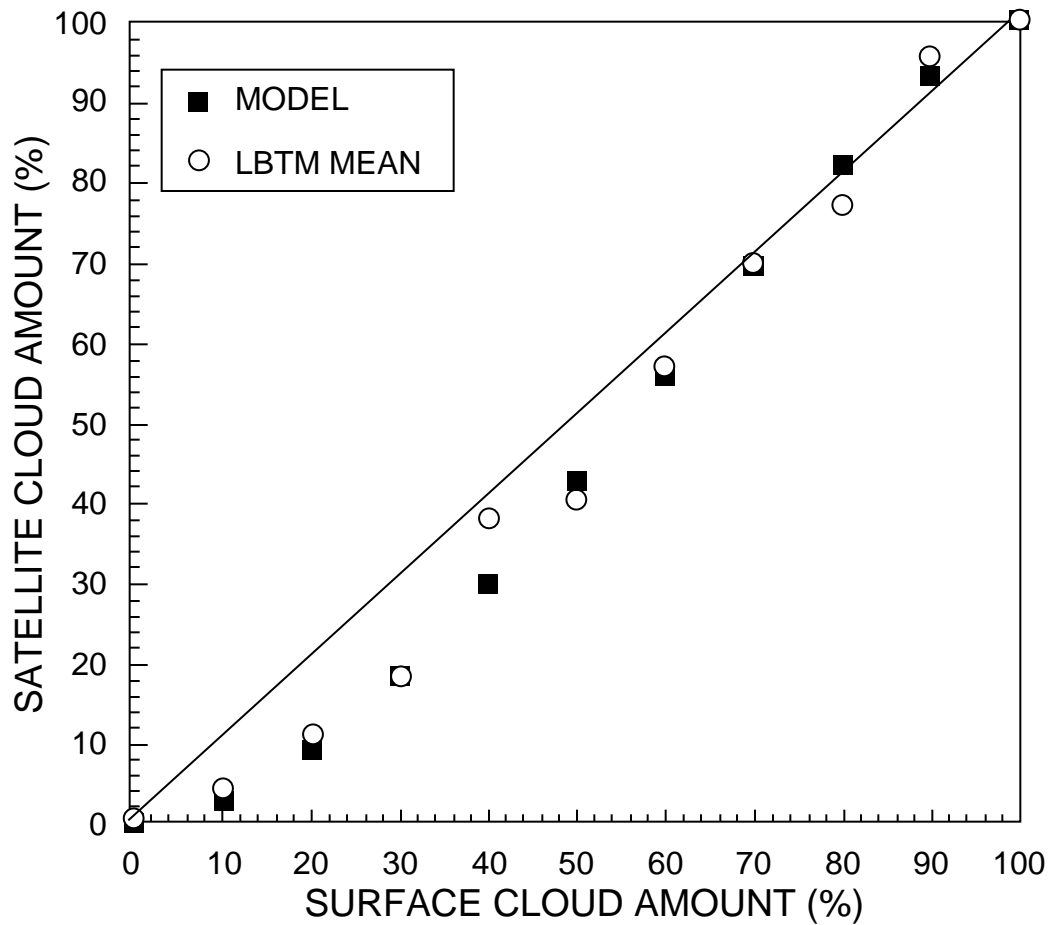
Figure 30. Mean satellite-observed cloudiness from WAFB and TAFB for each decile of surface-observed cloud fraction with an empirical model (eq. 24) based on whole-sky camera observations.
