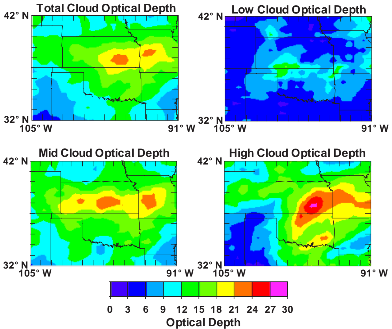
Figure 22. Mean cloud optical depths for 1330 to 2330 UTC for April 5 to May 1, 1994.
