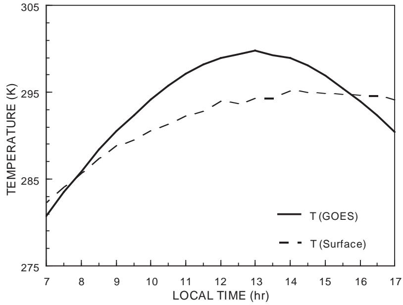
Figure 2. Mean hourly surface shelter and GOES-derived clear-sky temperatures for April 1994 over ARM SGP meso-scale domain.
