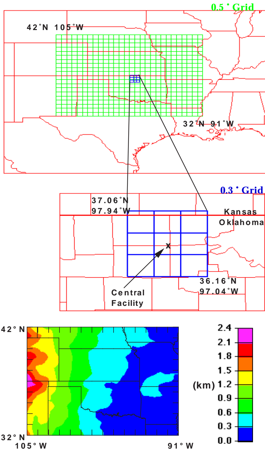
Figure 1. Satellite data analysis grids and surface elevation map for ARM Southern Great Plains locale.
