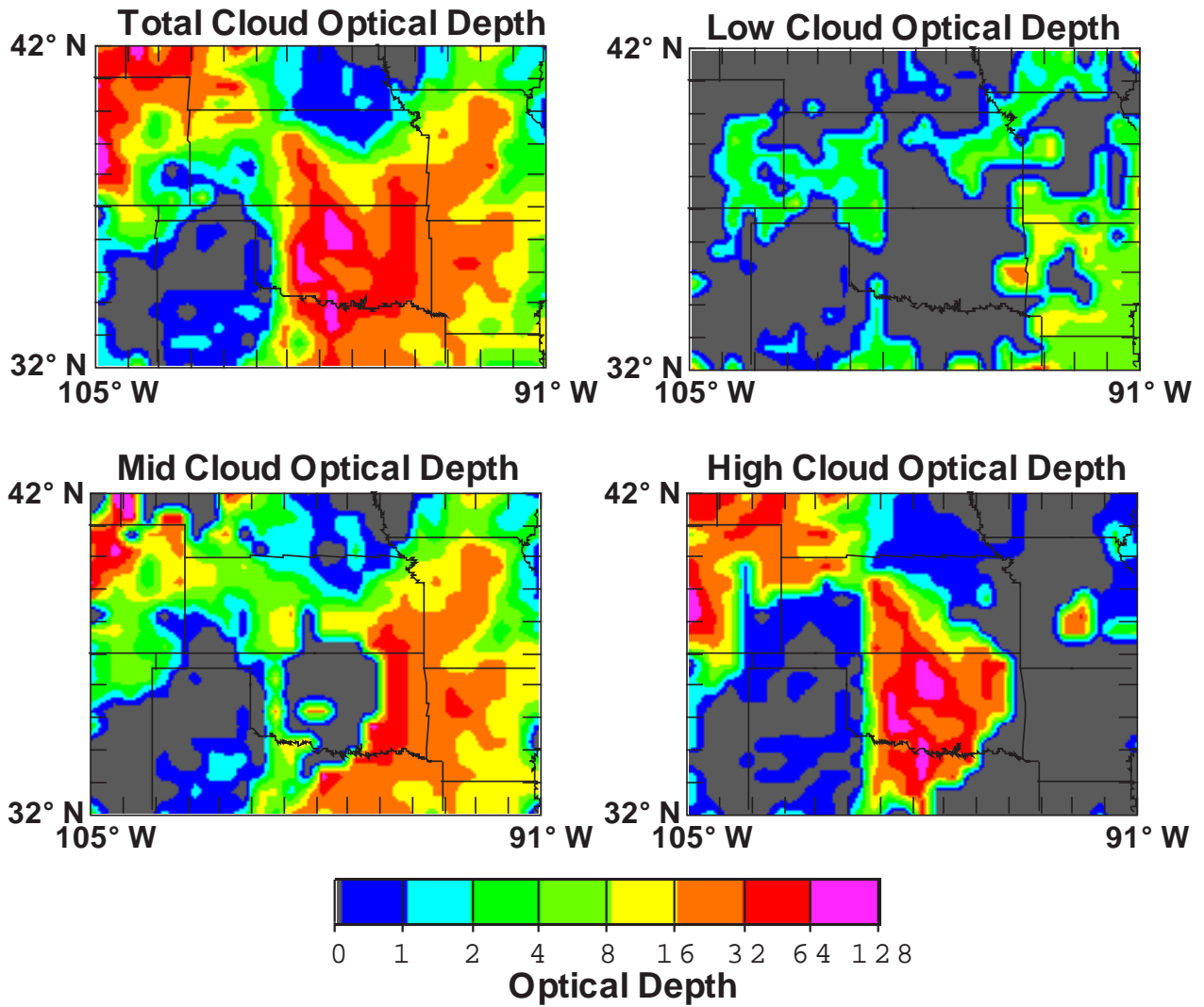
Figure 11. Cloud optical depths for 1800 UTC, April 25, 1994.
