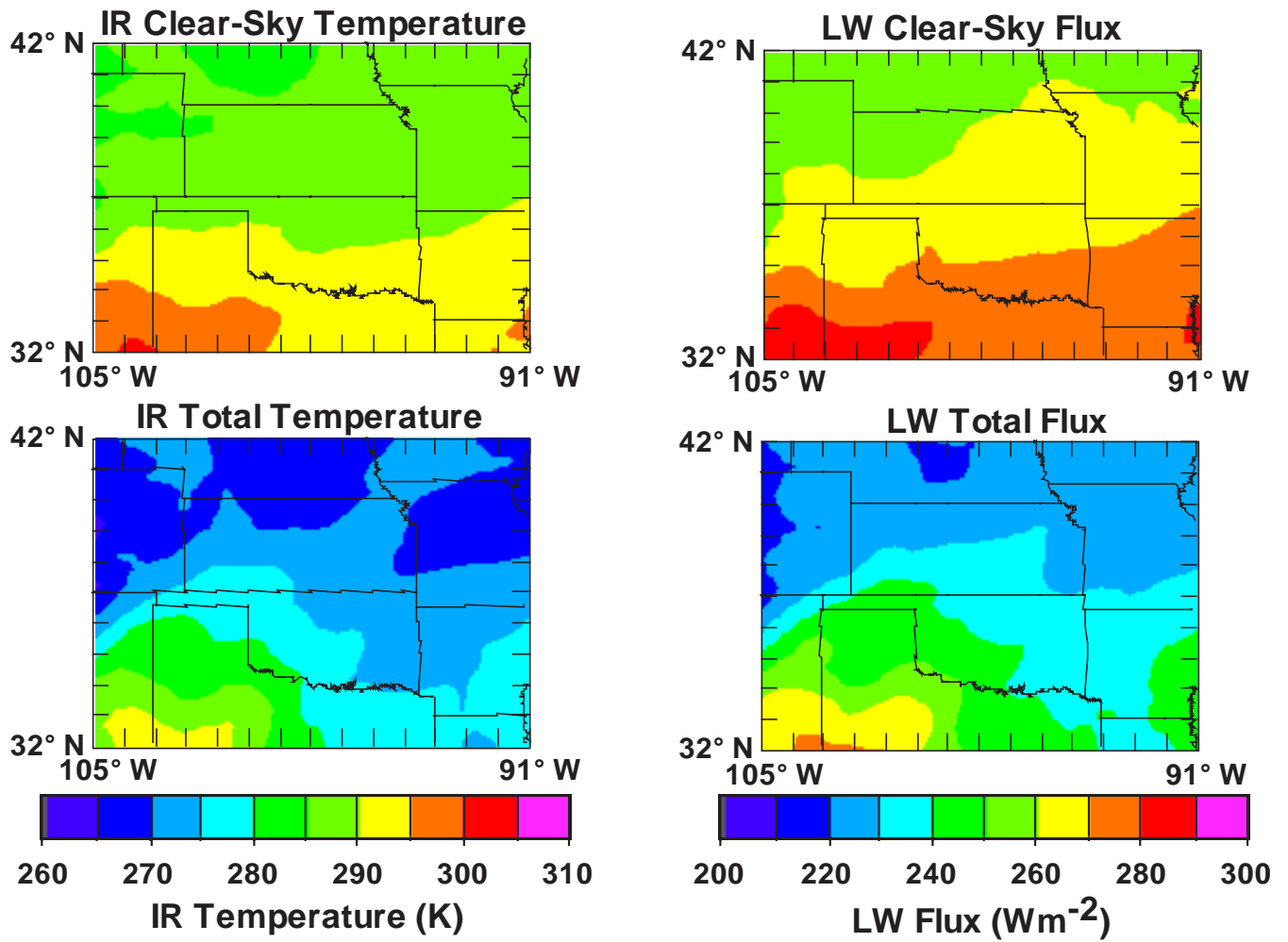
Figure 28. Mean IR temperatures and LW fluxes for 1330 to 2330 UTC for April 5 to May 1, 1994.
