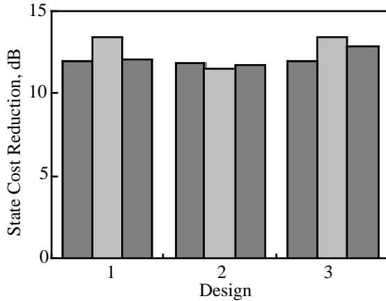
Figure 6 SISO Z axis control design performance on Configuration 1.
