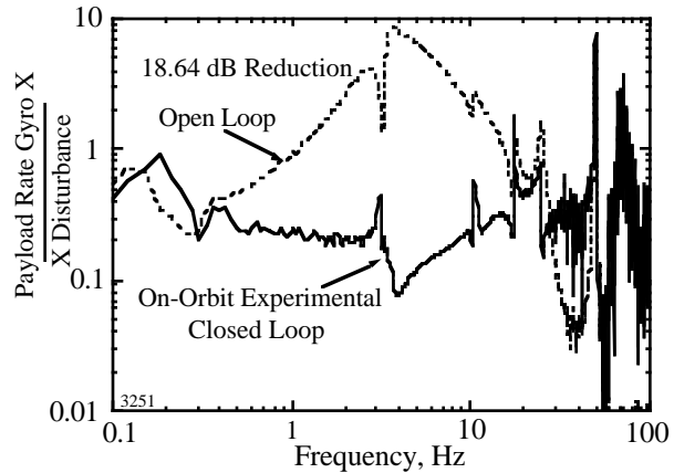
Figure 5 Open-loop vs closed loop performance for a SISO X axis control design on Configuration 1.
