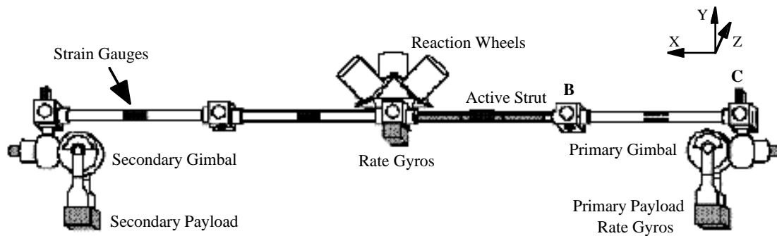
Figure 1 Middeck Active Controls Experiment (MACE) hardware sketch.
