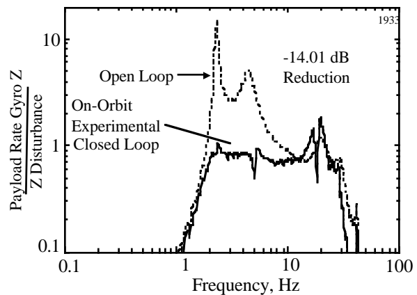
Figure 11 Open-loop vs. closed loop performance of a SISO Z axis control design for Configuration 2.
