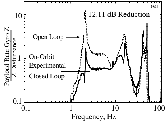
Figure 7 Open-loop vs closed loop performance of a SISO Z axis controller for Configuration 1.
