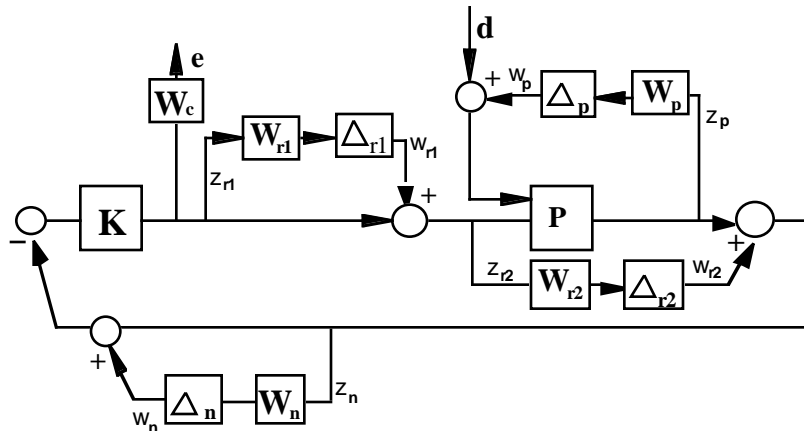
Figure 2 General H-infinity design structure showing uncertainties and weighting functions.
