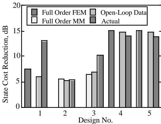
Figure 10 SISO Z axis control design performance on Configuration 2.
