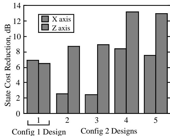
Figure 15 Actual performance of XZ axes control designs for Configurations 1 and 2.
