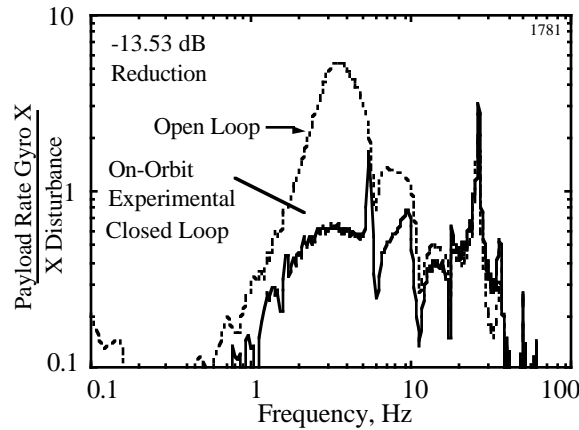
Figure 9 Open-loop vs. closed loop performance for a SISO X axis control design on Configuration 2.
