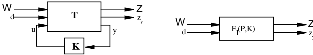
Figure 3 Linear fractional transformation of augmented plant matrix.
