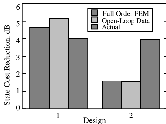
Figure 13 SISO Z axis control design performance for Reaction Wheel Z control only on Configuration 2.
