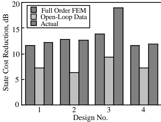
Figure 4 SISO X axis control design performance on Configuration 1.
