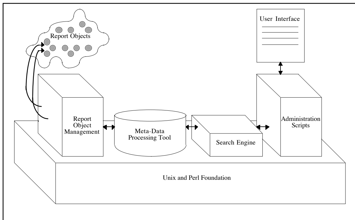
Figure 3. Intra-component communications.
