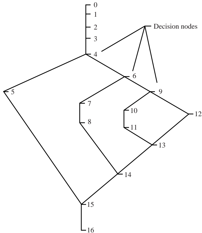
Figure 7. Structure graph for TSP functional unit.
