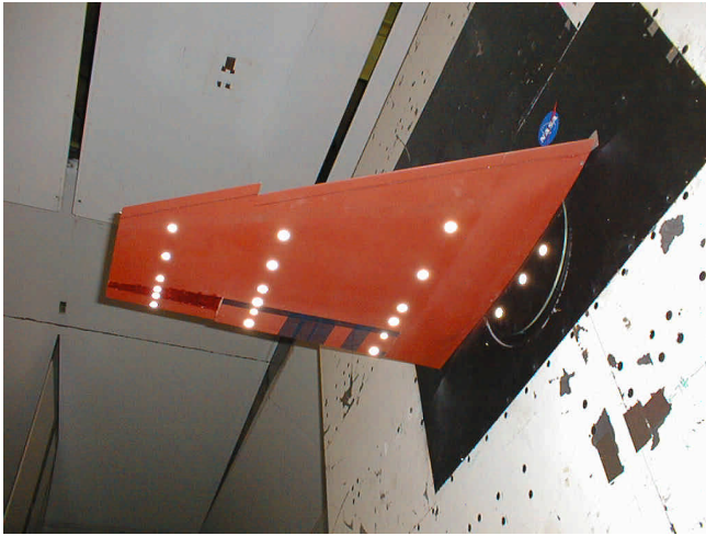
Figure 1: NGC Smart Wing with VMD targets at 22.7-, 61.2-, and 85.6-percent span.
