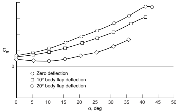
Figure 9. Reference Vehicle hypersonic pitching moment.
