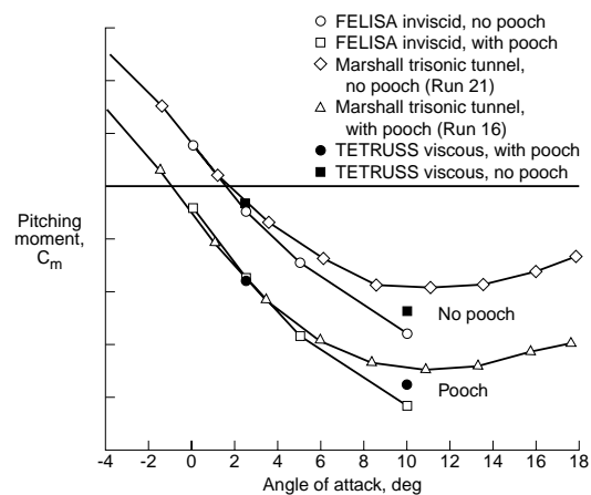
Figure 17. 0023 pooch vs. no pooch transonic pitching moment.
