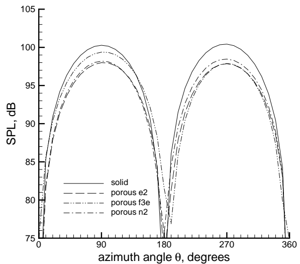
Figure 9.- SPL at 10 chords from source, fundamental frequency only, fine grid.
