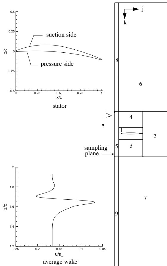
Figure 2.- Computational grid.
