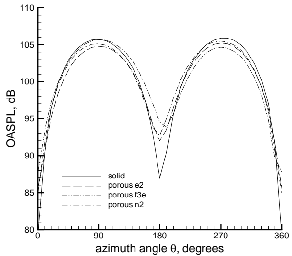
Figure 8.- OASPL at 10 chords from source, fine grid.
