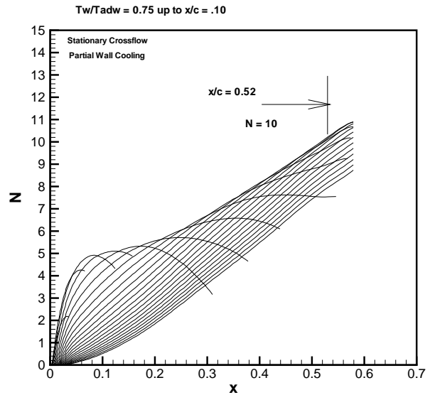
Fig. 17 N-factor vs. x/c for stationary crossflow for a Mach 2, 70° swept wing with T_w/T_{adw} = 0.75 for x/c < 0.1
