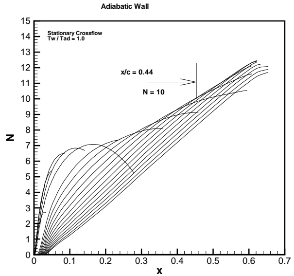
Fig. 16 N-factor vs. x/c for stationary crossflow for a Mach 2, 70° swept wing with an adiabatic wall condition
