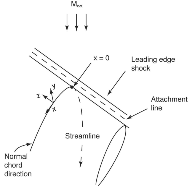
Fig. 2 Coordinate system for an infinite swept wing boundary layer
