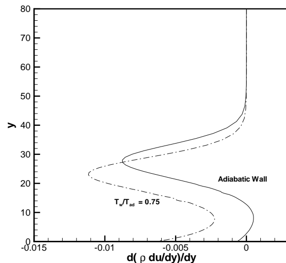
Fig. 14 Generalized inflection point for the streamwise velocity component for an adiabatic and cooled wall, Mach 2 infinite swept wing boundary layer
