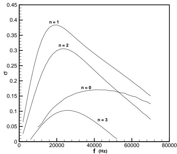
Fig. 13 Growth rates vs. disturbance frequency for the Mach 2.5 jet at x = 0.02 m for different azimuthal wave numbers
