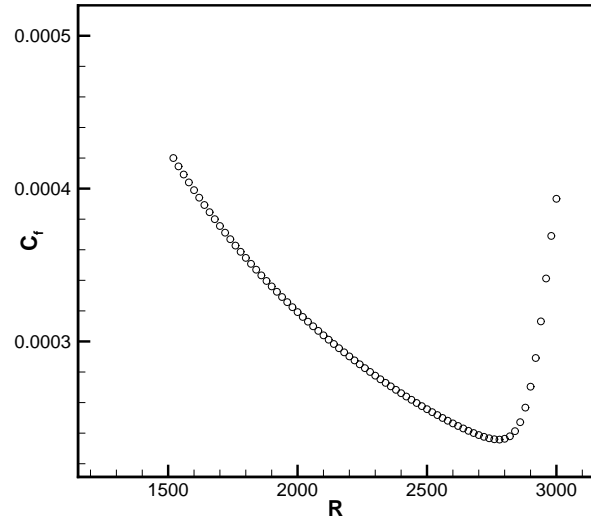
Fig. 7 Skin friction coefficient vs. Reynolds number for a Mach 2 flat plate boundary layer undergoing an oblique-mode breakdown
