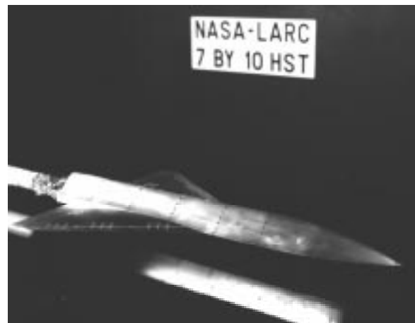
Figure 4. Installation of 30° chine angle fuselage configuration in the Langley 7-by-10-Foot HST.
