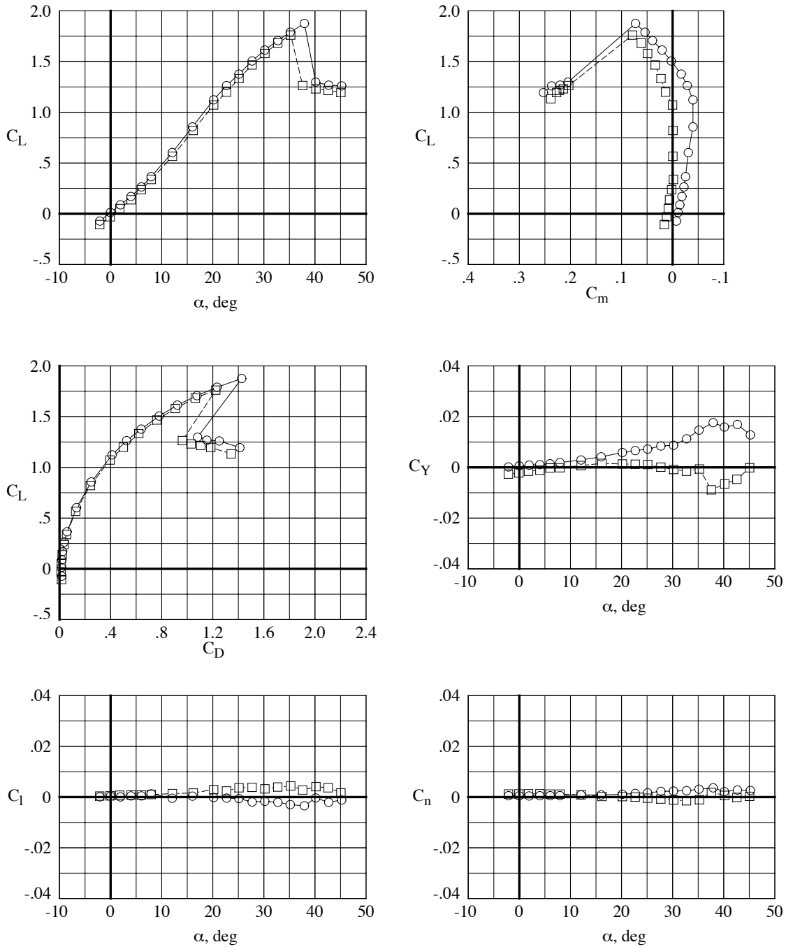
Figure 5. 30° chine fuselage. Force and moment data for upright and inverted configurations. \beta = 0^\circ .
