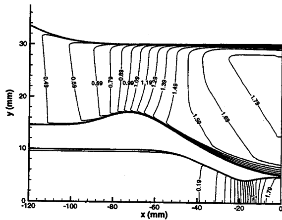
Figure 3 SPARK code calculation of Mach number.
