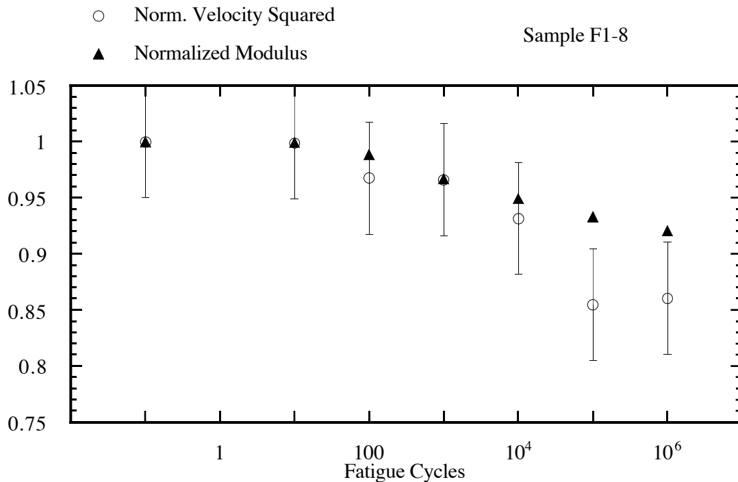
Figure 3. Normalized velocity squared vs. fatigue cycles for sample F1-8.
