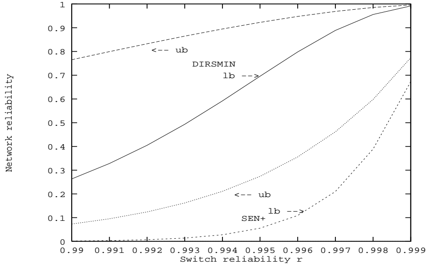
Figure 12: All-terminal reliability bounds for DIRSMIN and SEN+. N = 64 and r = \text{variable}
