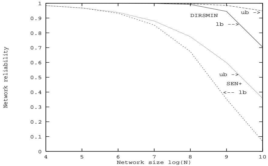
Figure 13: All-terminal reliability bounds for DIRSMIN and SEN+. r = 0.999 .
