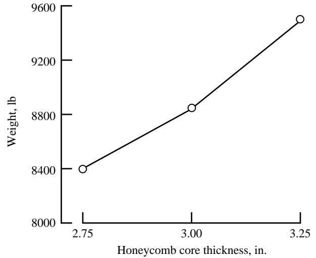
Figure 15. Weight sensitivity of honeycomb core thickness.
