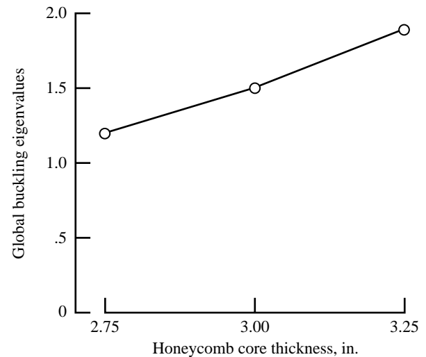
Figure 16. Global buckling sensitivity of honeycomb core thickness.
