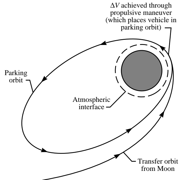
Figure 1. Propulsive capture.
