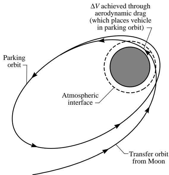
Figure 3. Aerodynamic capture.
