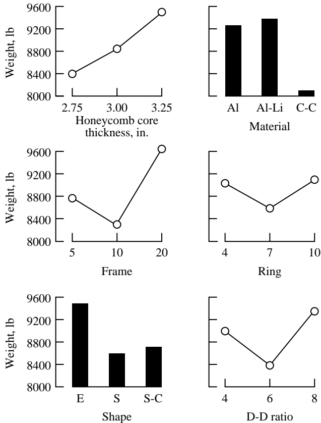
Figure 13. Response graphs.
