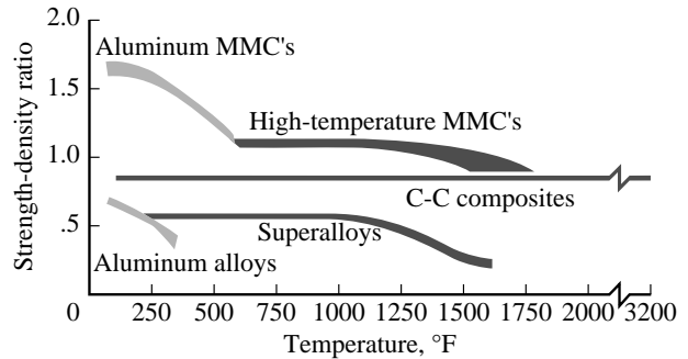
Figure 6. Temperature performance of materials.
