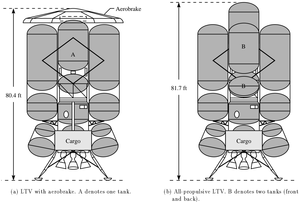
Figure 2. Lunar transfer vehicle configurations (ref. 4).
