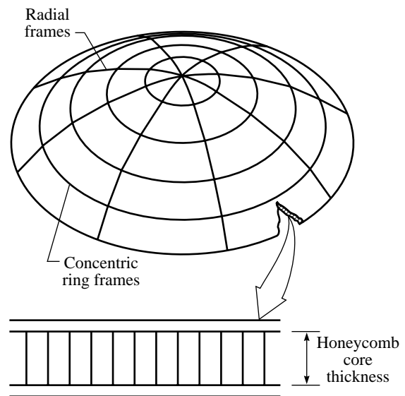
Figure 4. Concentric ring frames (rings), radial frames (frames), and honeycomb core thickness.
