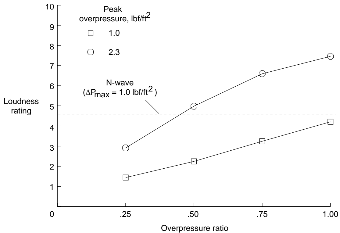
Figure 5. Subjective loudness as function of overpressure ratio for each front-shock rise time and for peak overpressures of 1.0 and 2.3 lbf/ft 2 .
