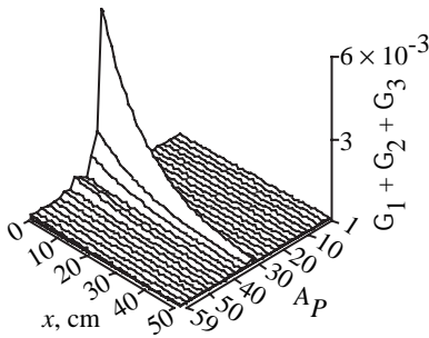
Figure 9. Total ^{28}\text{Si} production from first three collisions.
