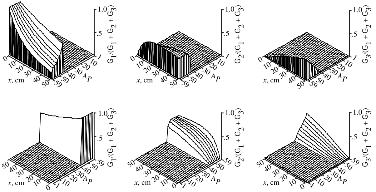
(a) First collision. (b) Second collision. (c) Third collision.
