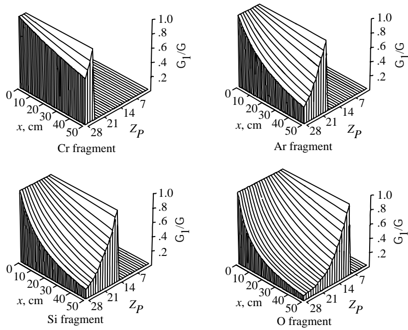
Figure 14. Fraction contribution of first collision term of specific elements.
