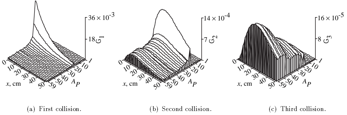
Figure 10. First three collision contributions to ^{16}\text{O} production.
