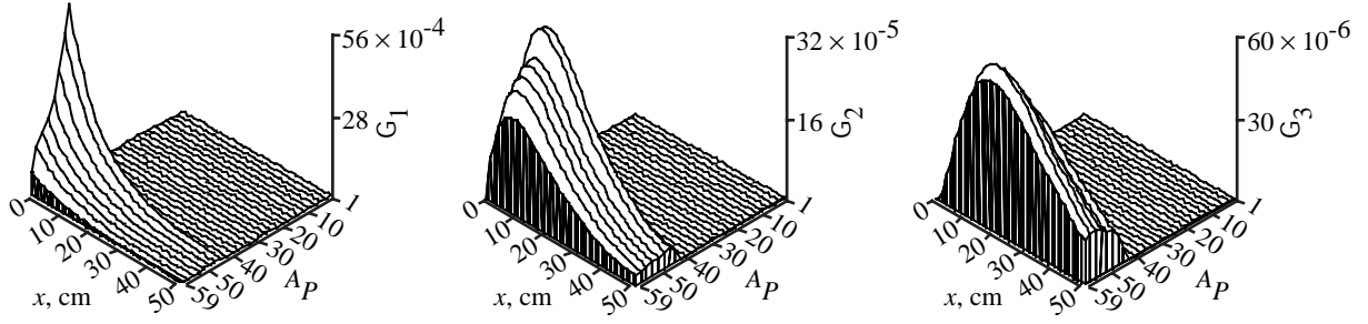
(a) First collision. (b) Second collision. (c) Third collision.
