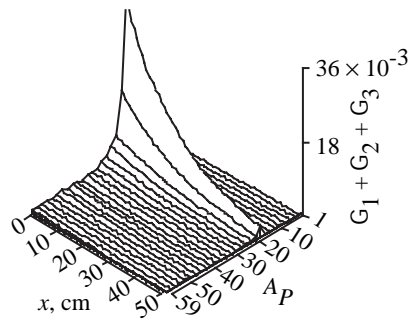
Figure 12. Total ^{16}\text{O} production from first three collisions.
