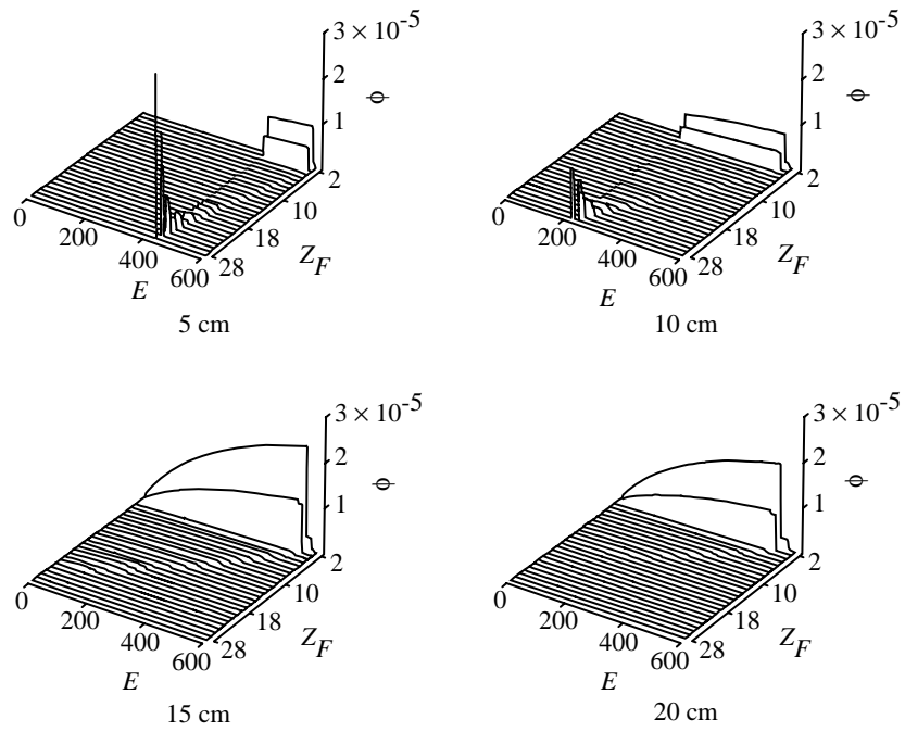
Figure 15. Composition of a 535 MeV/nucleon iron beam in a water column.
