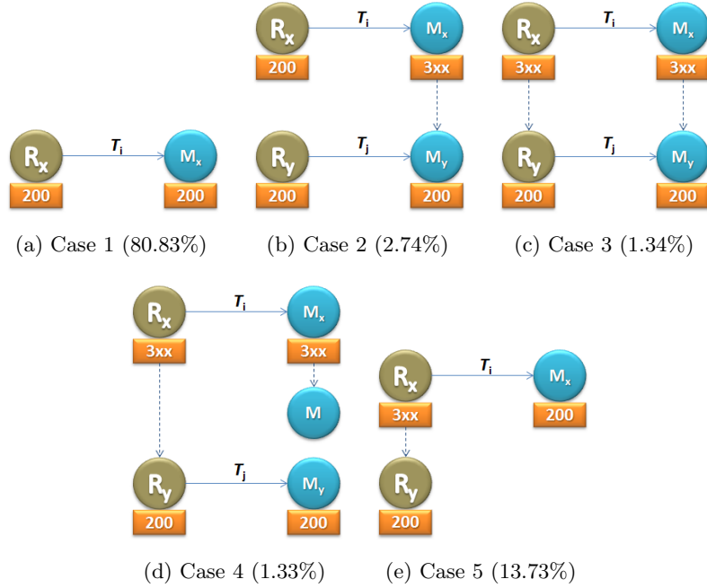
Figure 2: URI-R & URI-M HTTP Redirection relationship cases.
