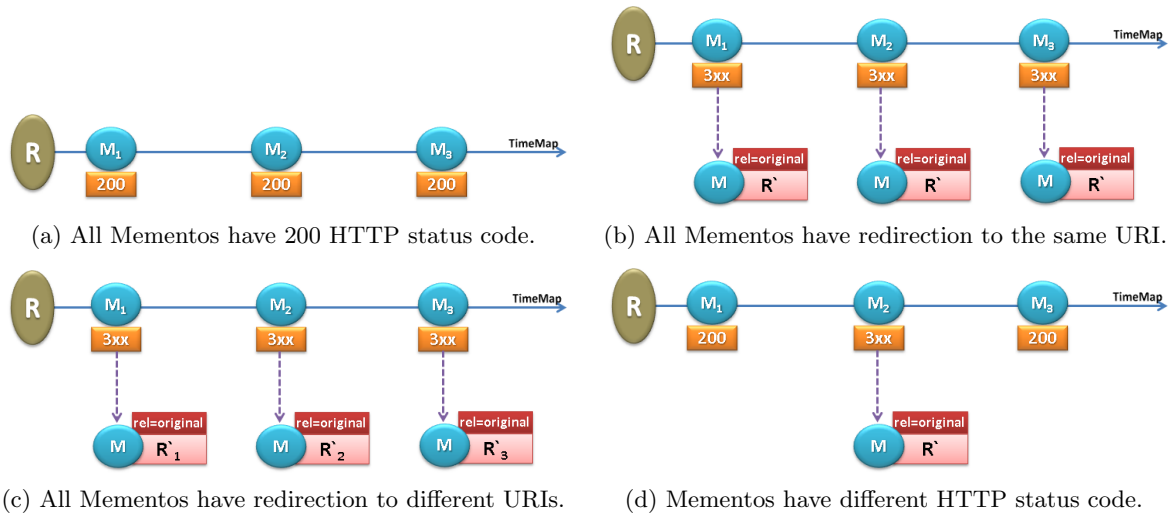
Figure 1: Timemap Redirection Categories.
