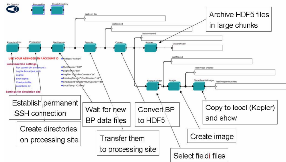
Figure 1. A Kepler-based workflow
